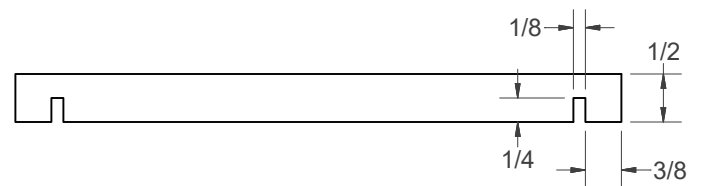
UPPER AND LOWER RACK (8) SCALE 1
