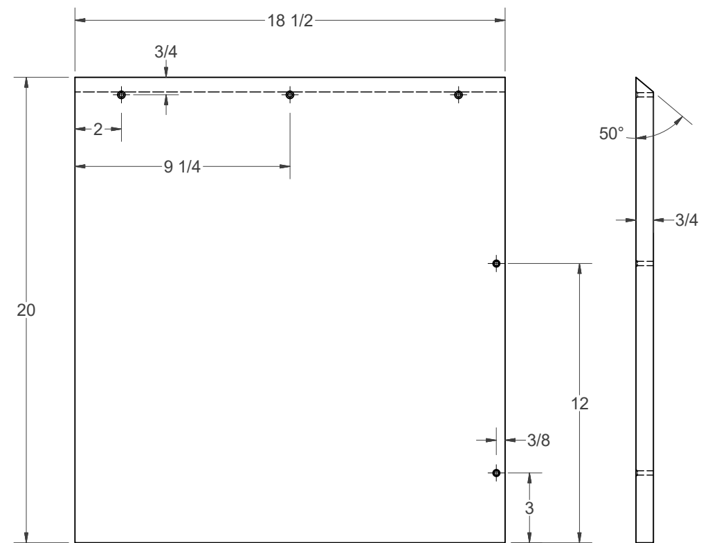
DUST FUNNEL SIDES (2) SCALE .35
