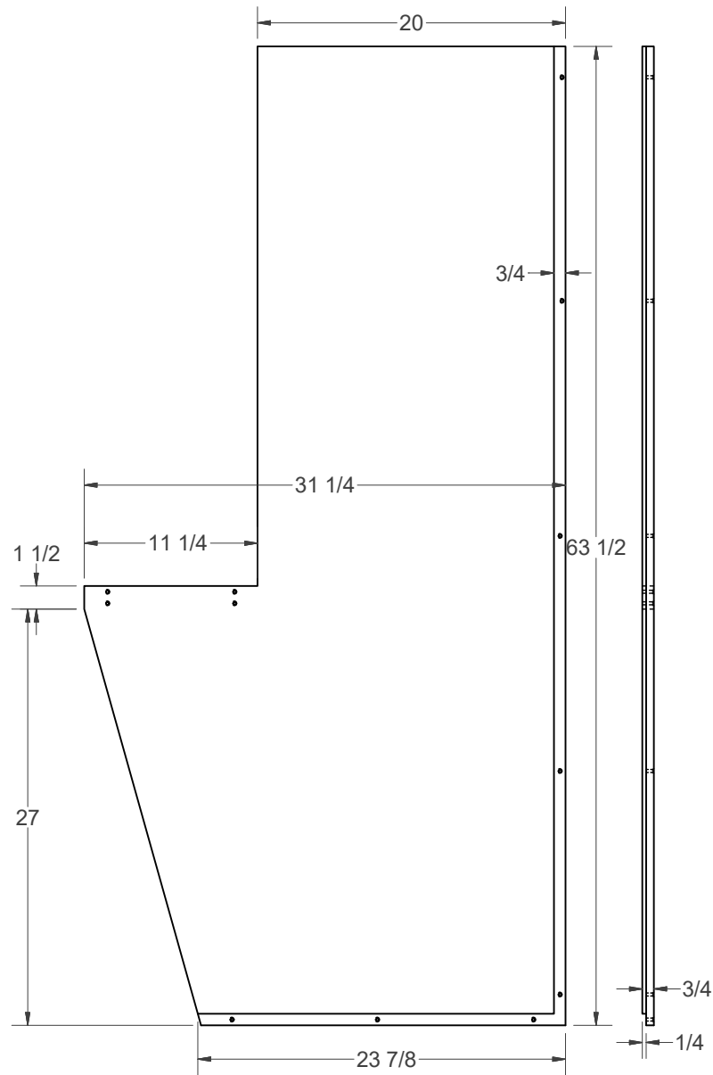
LEFT SIDE (1) SCALE .18
