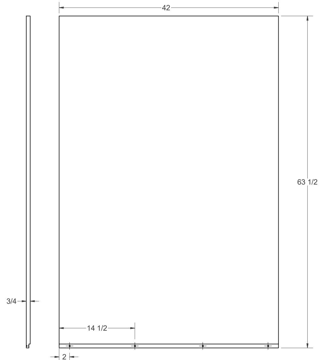
BACK (1) SCALE .18
