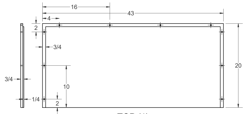
TOP (1) SCALE .18
