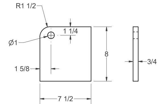
REAR PIVOT BRACKET (2) SCALE .25
