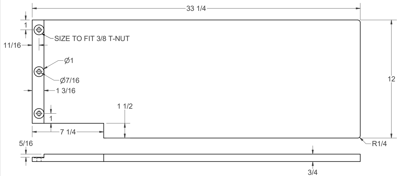
RIGHT WING TOP (1) SCALE .35
