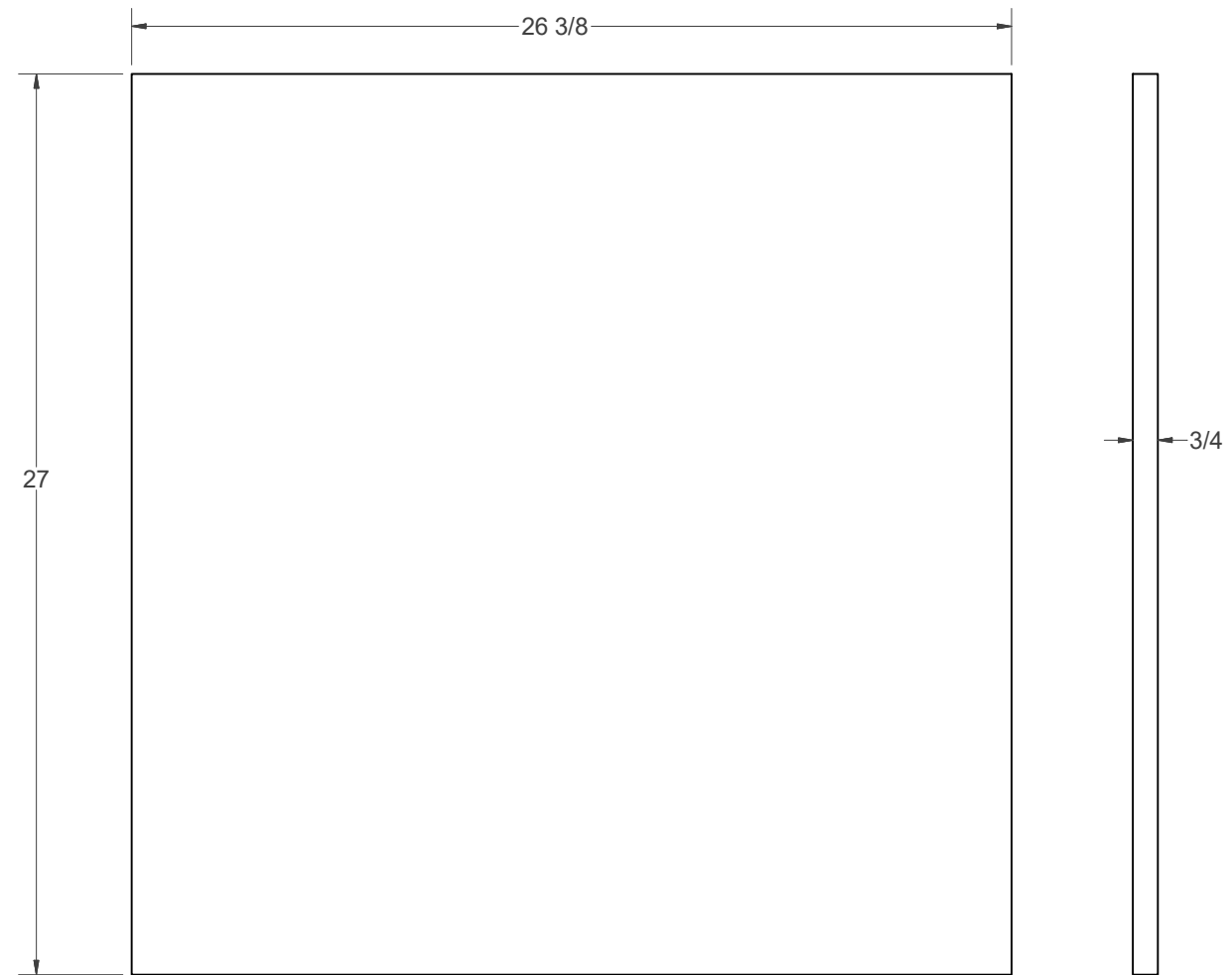
ACCESS PANEL SCALE .35
