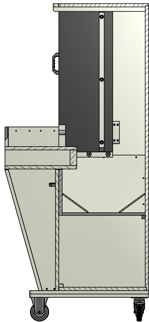
SECTION D-D SCALE .15
