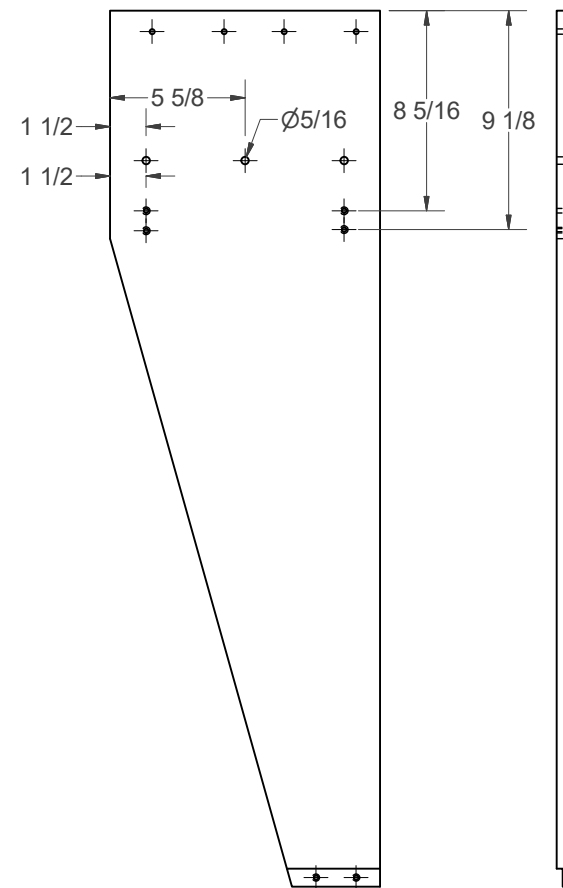
RIGHT POST SIDE (1) SCALE .25
