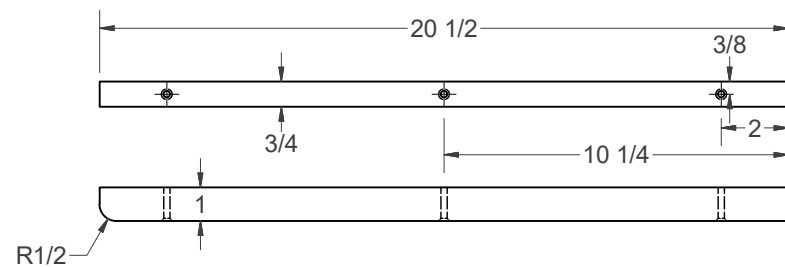
WING GUIDE STRIP (2) SOLID WOOD SCALE .35
