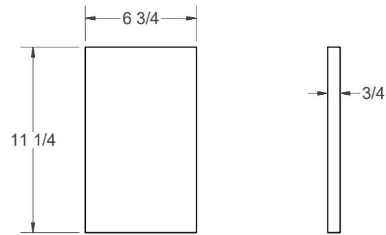
POST CAP (4) SCALE .25
