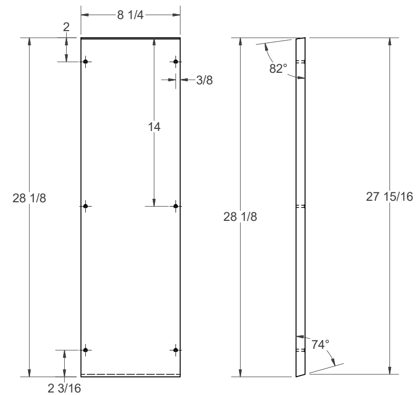
POST FACING (2) SCALE 1 / 4
