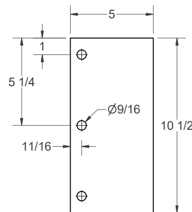
WING WIDE FILLER (2) SOLID WOOD SCALE .35
