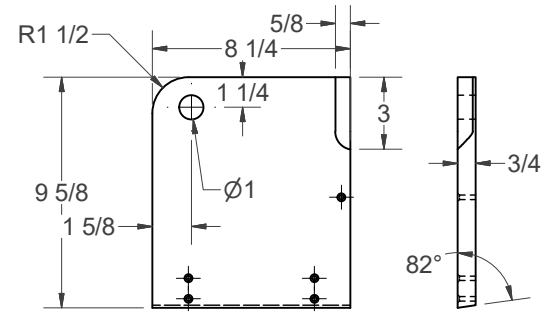
FRONT PIVOT BRACKET-LEFT (1) SCALE .25
