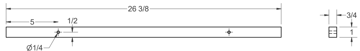
ACCESS PANEL LEDGER SCALE .35
