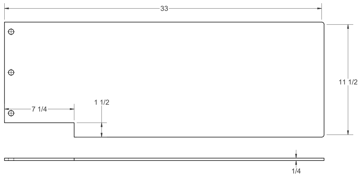
RIGHT WING BOTTOM (1) SCALE .35
