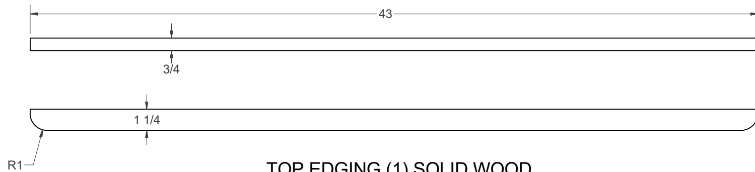
TOP EDGING (1) SOLID WOOD SCALE .35
