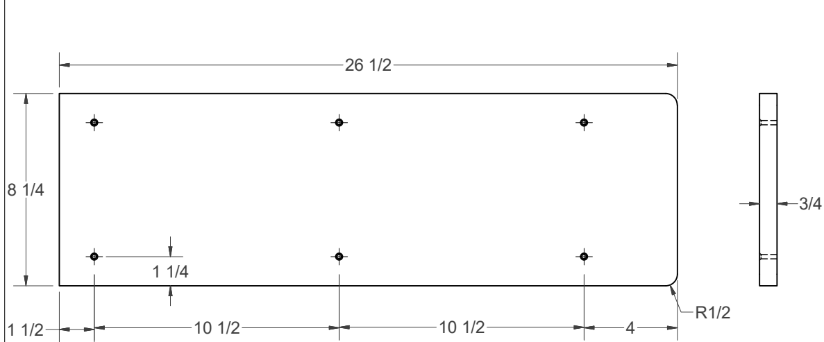
CASTOR PLATE (4) SCALE .35
