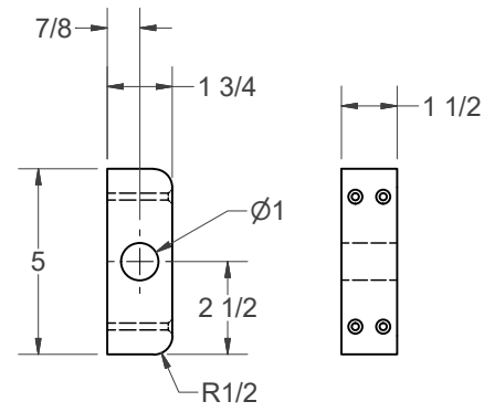
ROD BRACKET (2) SOLID WOOD SCALE .35
