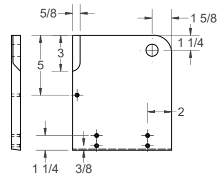
FRONT PIVOT BRACKET-RIGHT (1) SCALE .25
