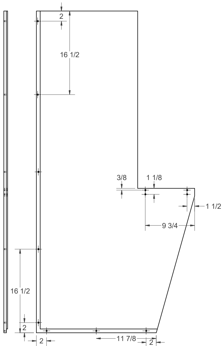
RIGHT SIDE (1) SCALE .18
