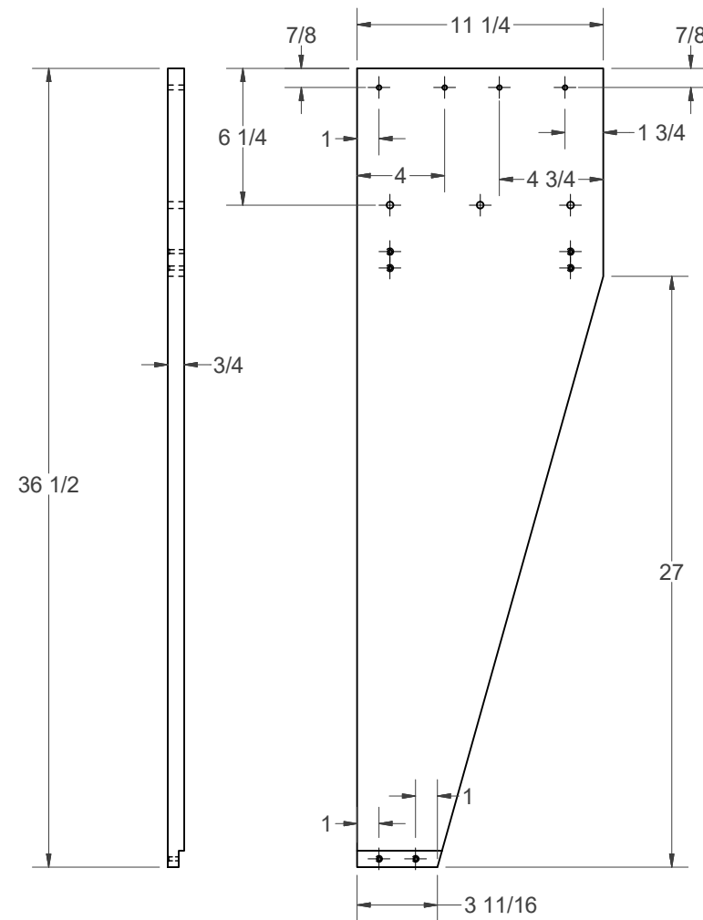
LEFT POST SIDE (1) SCALE .25
