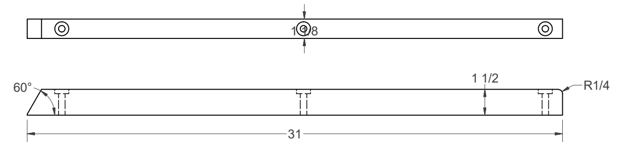
FENCE SCALE .35
