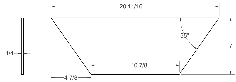
DUST FUNNEL KICKERS (2) SCALE .35
