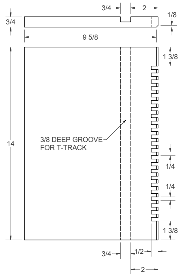
(O) - INDEXING PLATE
