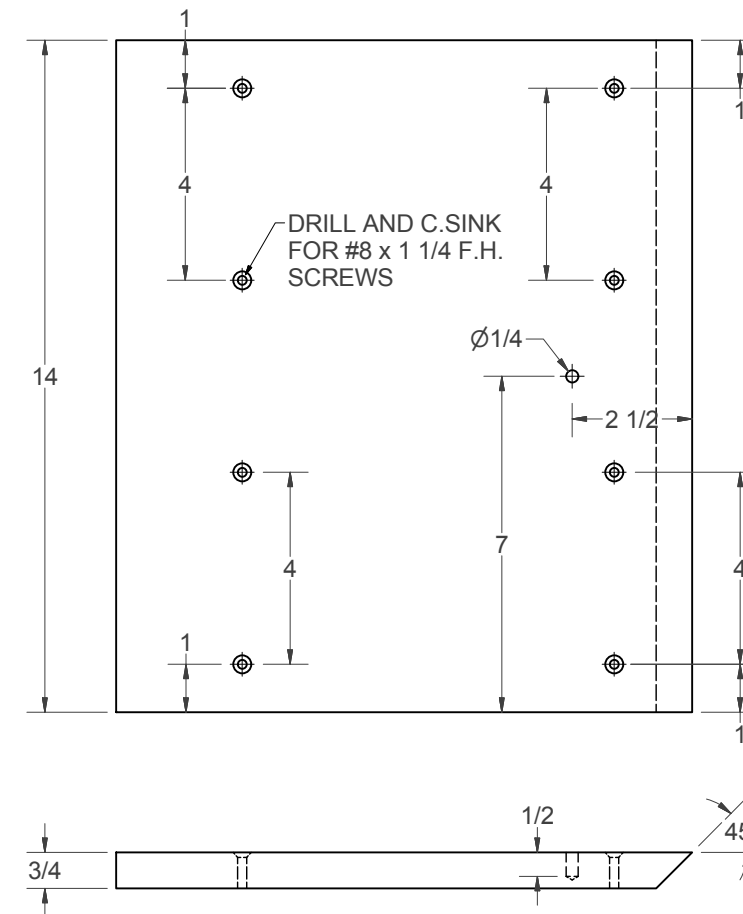
(M) - MOUNTING BAR
