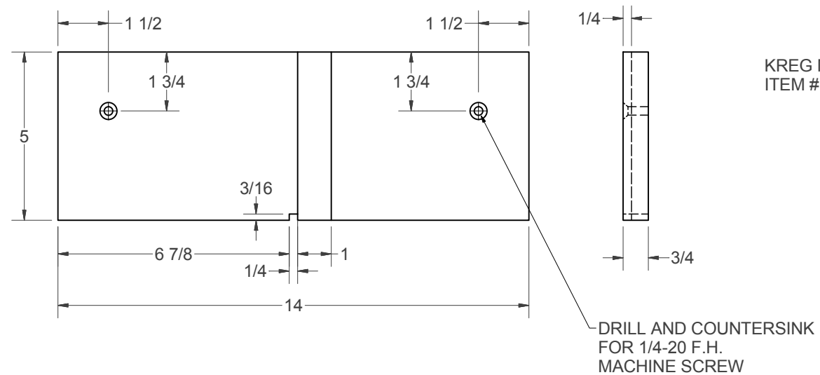
(F) - BOX JOINT BACK PLATE
