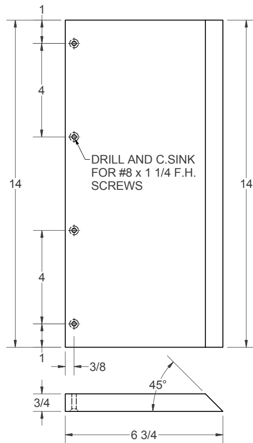
(J) - SLOT JIG BASE
