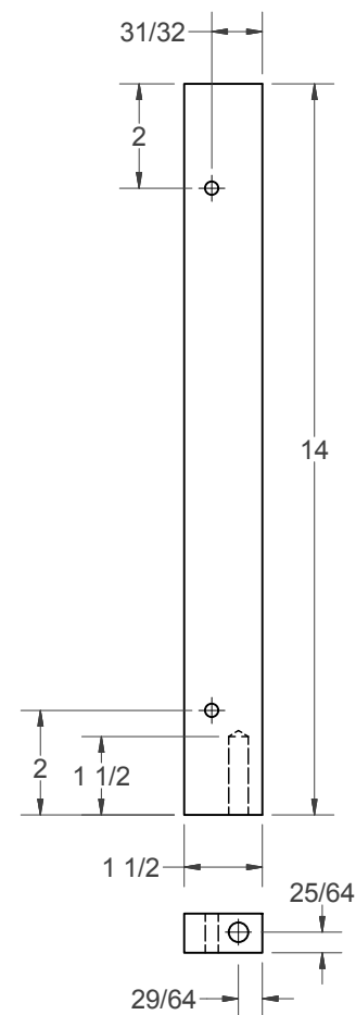
(M) - MOUNTING BAR
