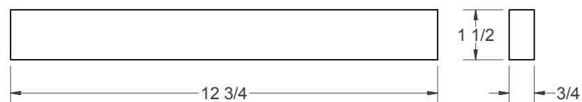
(P) - CLEAT
