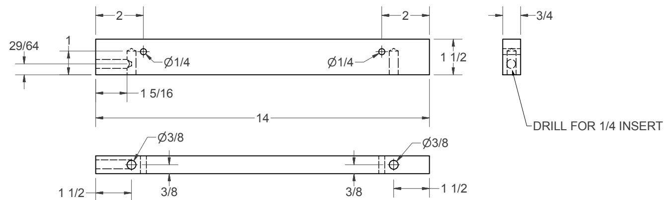
(G) - BOX JOINT MOUNTING BAR
