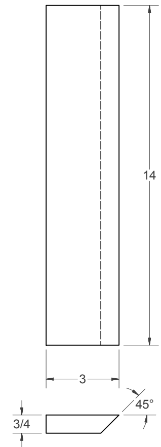
(N) - INDEXING RAIL
