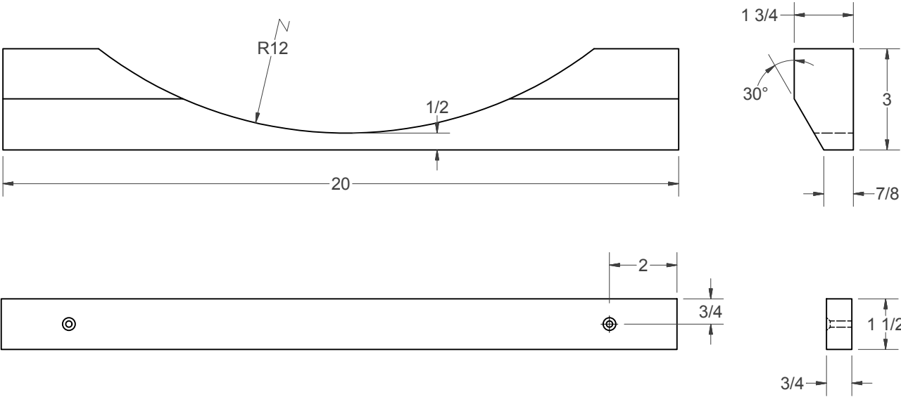
SEAT TRIMMING JIG
