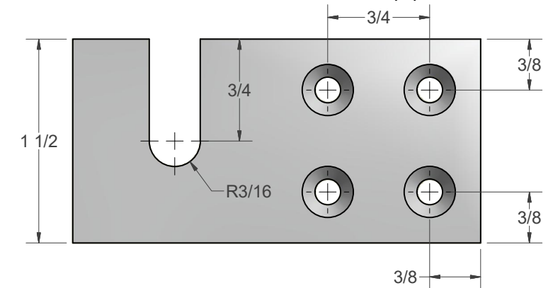
RIGHT RAIL BRACKET (3)
