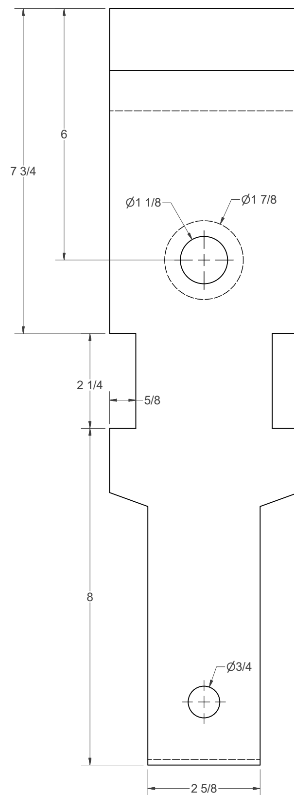
(A) - REAR JAW - FRONT
