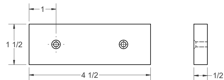
(C) - JAW FACES
