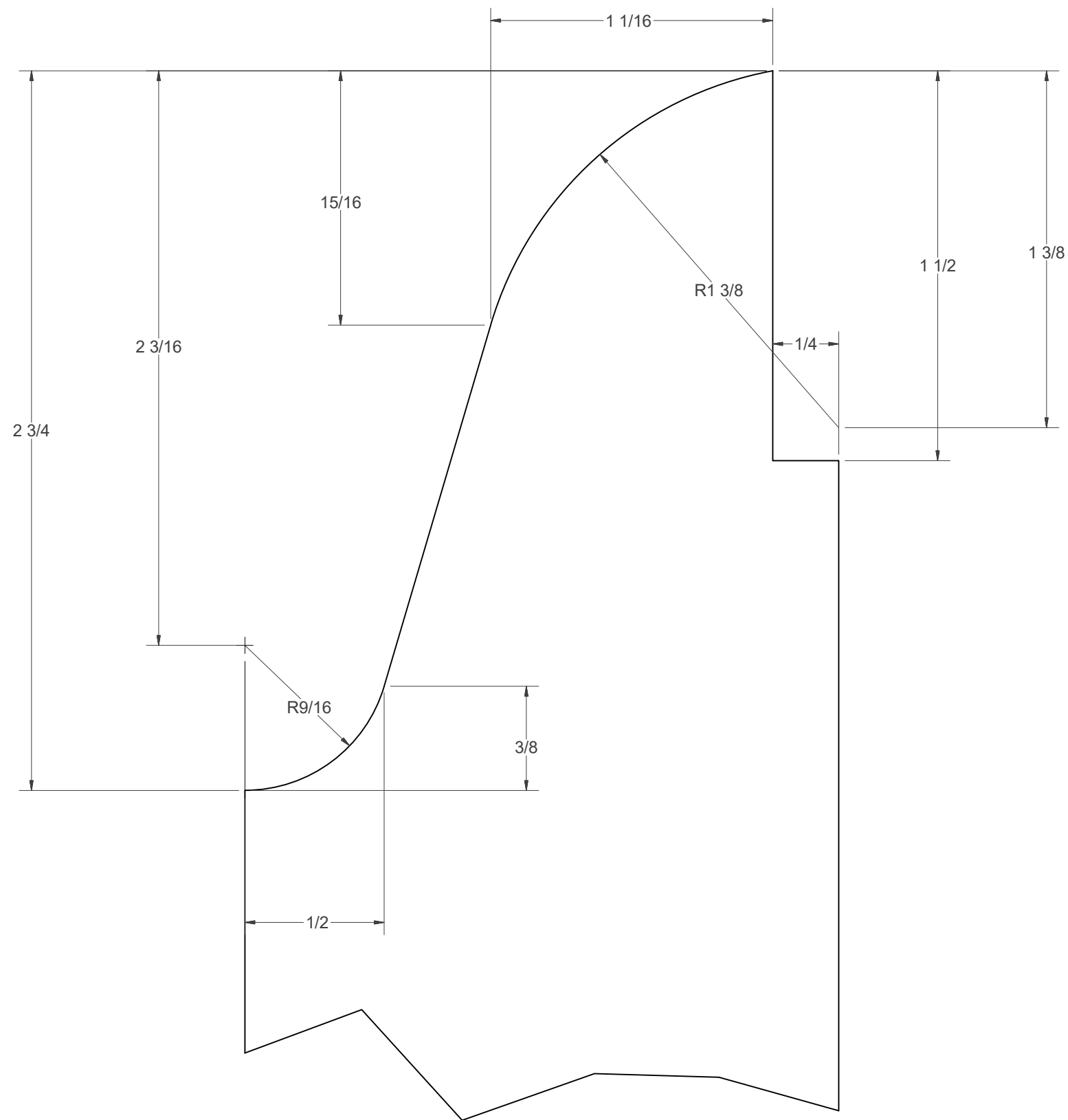
DETAIL E
