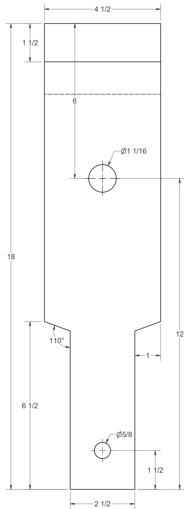
(A) - FRONT JAW
