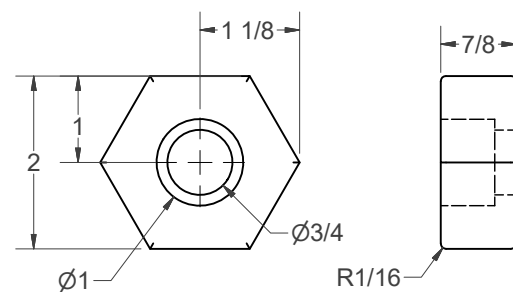
(G) - STOP NUT
