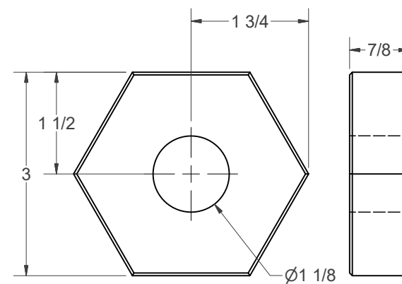
(H) - BENCH NUT
