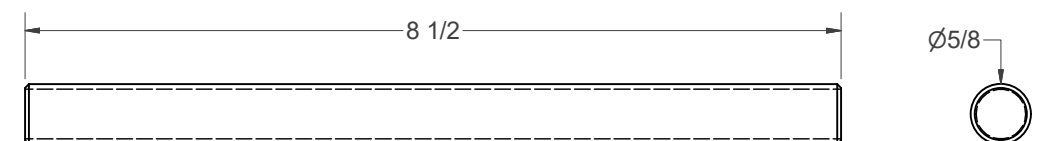
ADJUSTER (5/8" ACME ROD)
