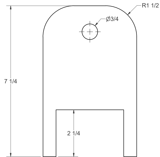
(B) - BRACKET
