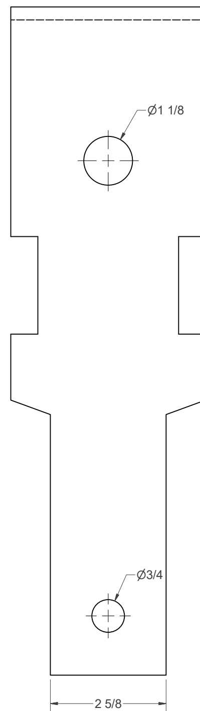
(A) - REAR JAW - BACK
