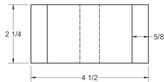
(B) - BRACKET
