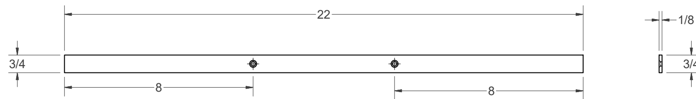
LONG LOCK BAR - 1/8" X 3/4" ALUMINUM
