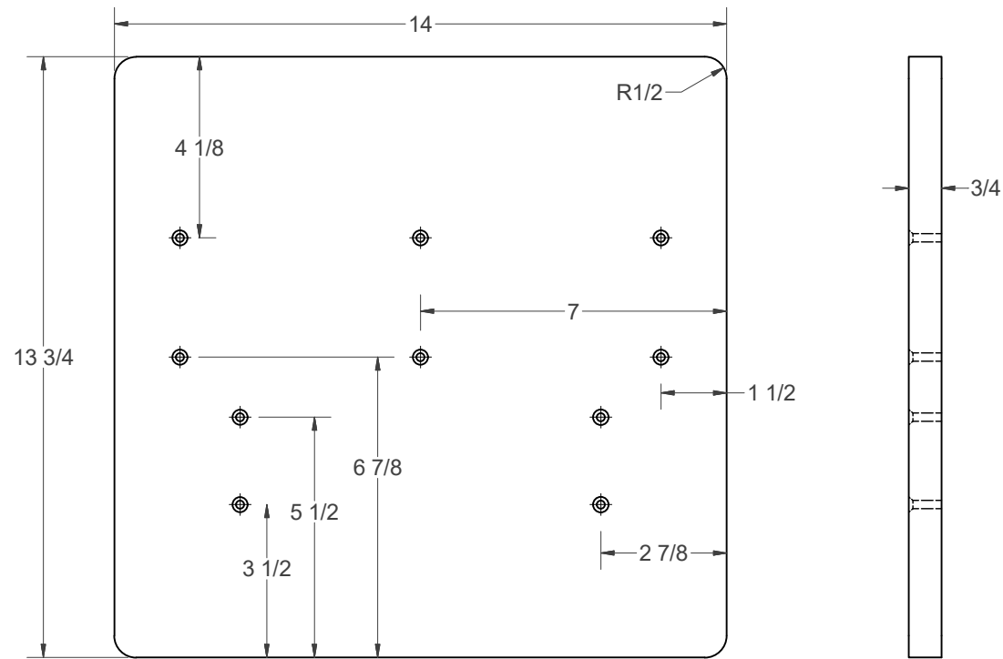
OUTFEED BASE - 3/4" PLYWOOD
