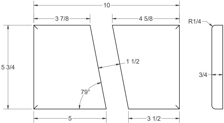
RIGHT AND LEFT LEG BRACKET - 3/4" PLYWOOD (NEED 4)
