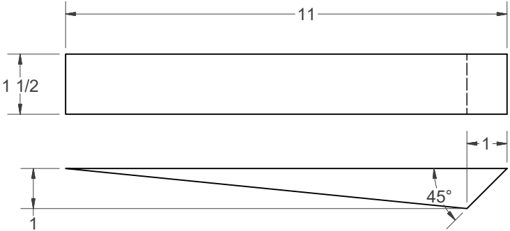
TENSION WEDGE - SOLID WOOD (NEED 2)
