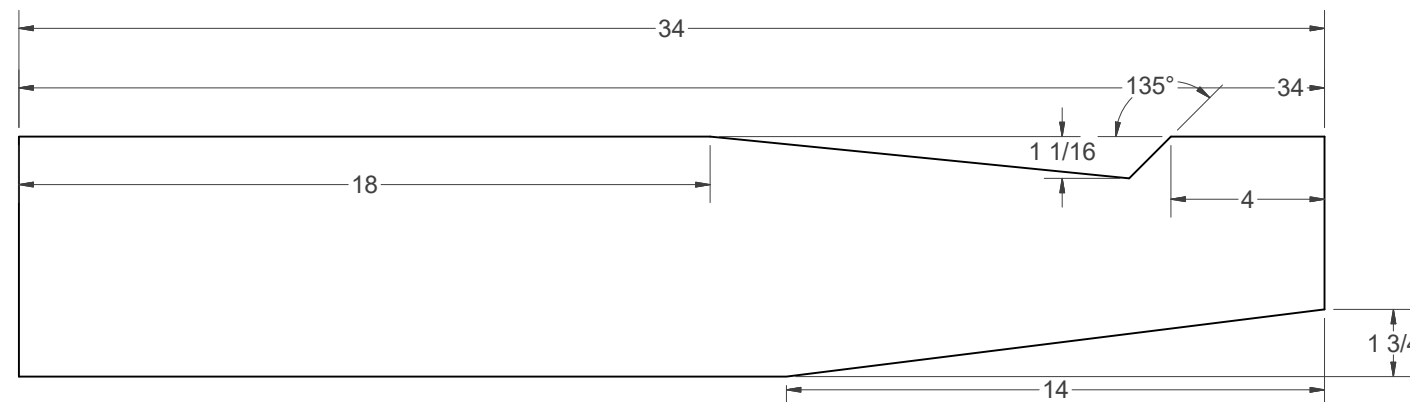
LOCKING ARM 1 1/2" PLYWOOD
