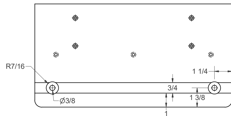
FRONT - 3/4" PLYWOOD
