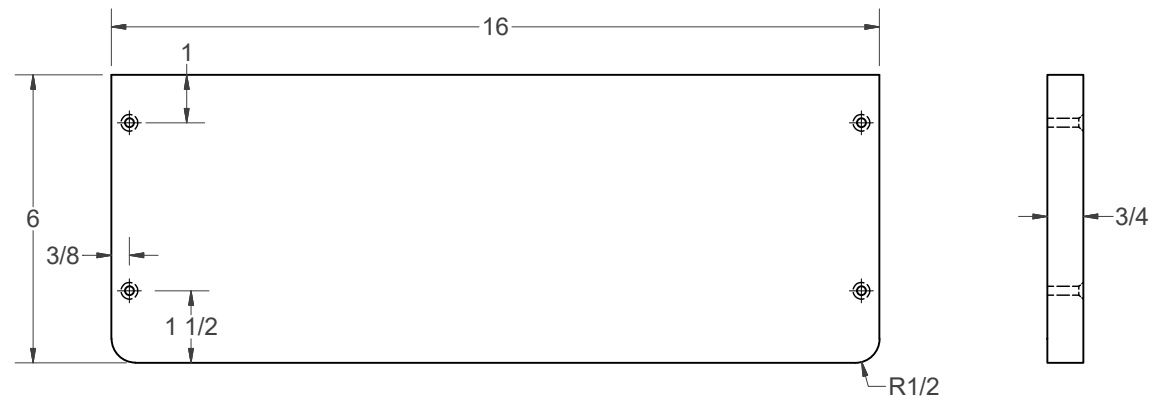
SHELF - 3/4" PLYWOOD
