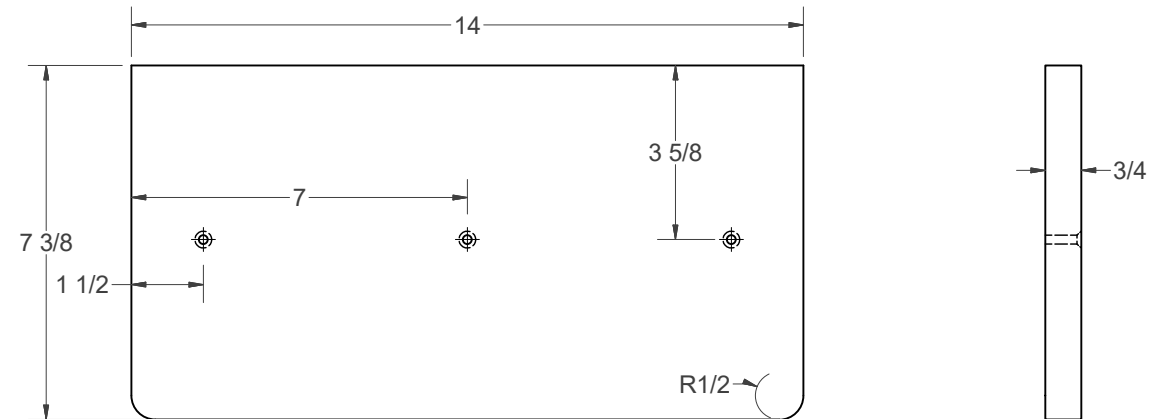
BACK - 3/4" PLYWOOD
