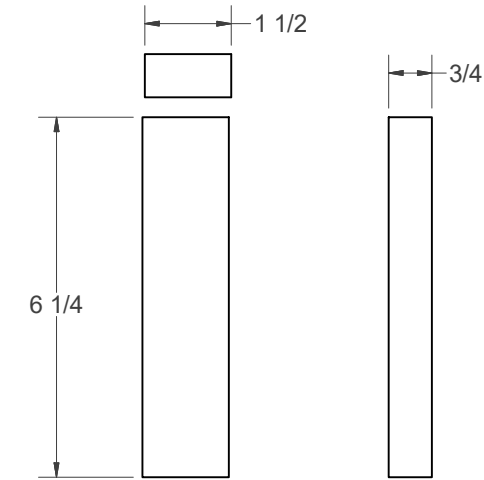
FILLER - 3/4" SOLID WOOD (NEED 4)
