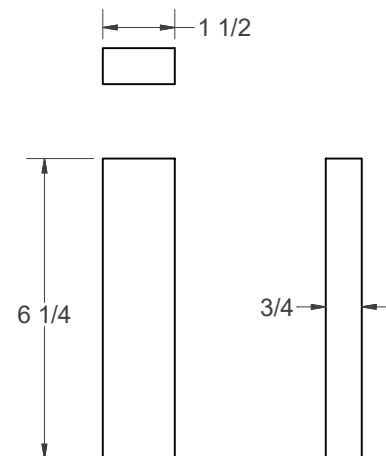
FILLER - 3/4" SOLID WOOD (NEED 2 PER EXTENSION BEAM)
