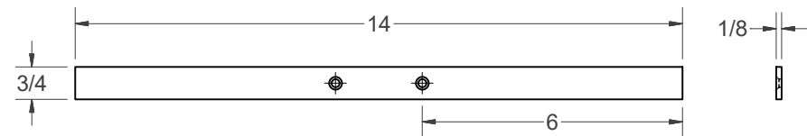
SHORT LOCKING BAR - 1/8" X 3/4" ALUMINUM
