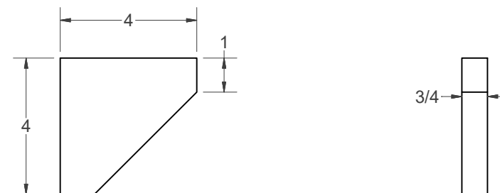
BRACE - 3/4" PLYWOOD (NEED 2 PER OUTFEED PLATFORM)
