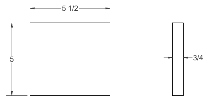
SIDE - 3/4" PLYWOOD (NEED 2)
