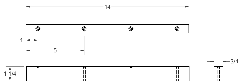
FENCE - 3/4 " SOLID WOOD
