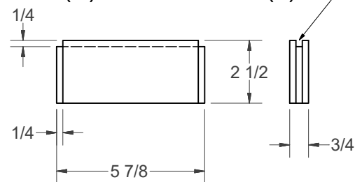
(Y) - DOOR RAIL (2)
