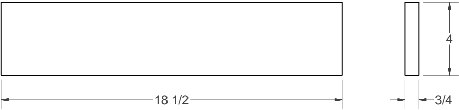
(J) - UPPER RAIL (2)
