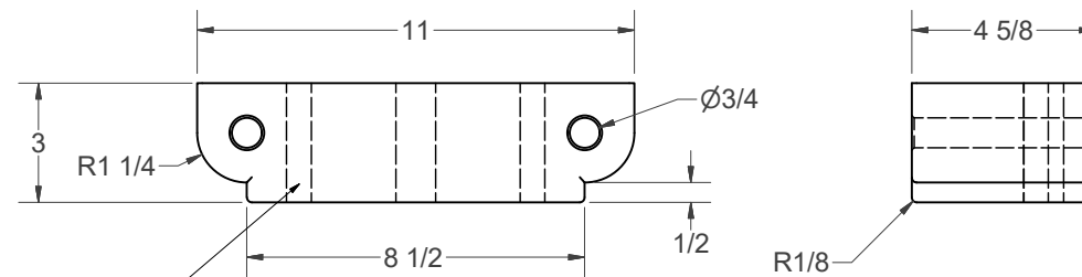
(DD) - VISE JAW (GLUED UP FROM 3/4 MATERIAL)
