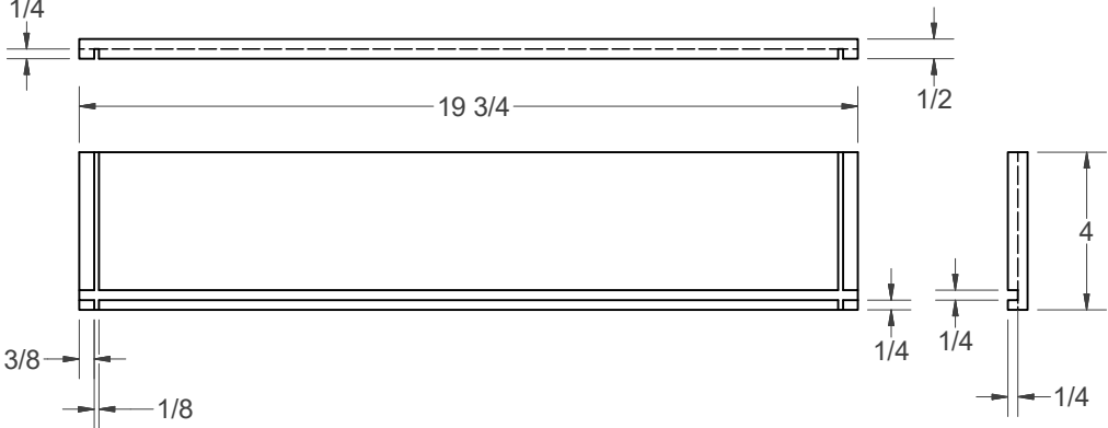
(R) - DRAWER SIDE (6)
