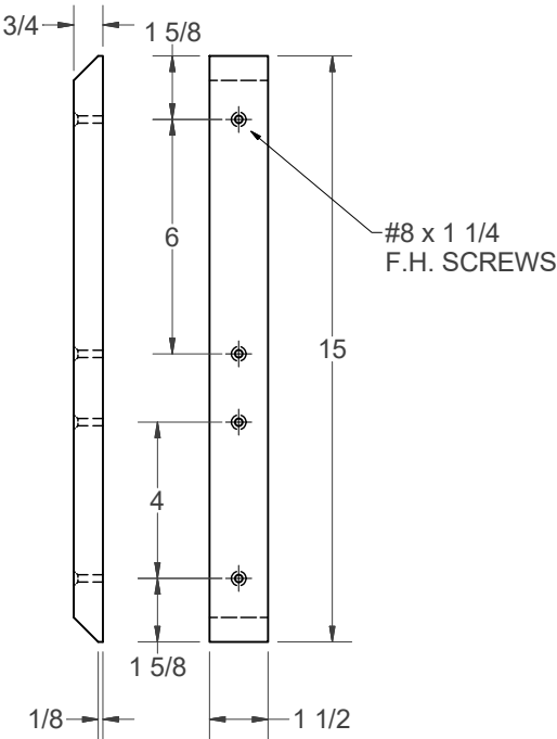
(II) - RACK SUPPORT (2)
