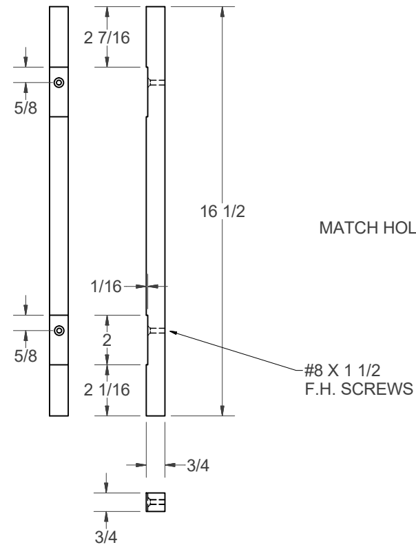
(X) - DOOR HANGING STILE
