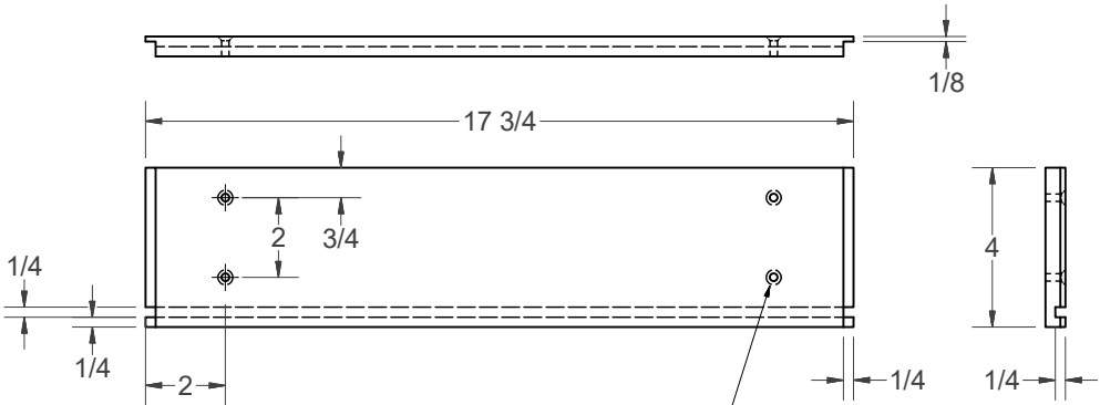
(S) - DRAWER FRONT/BACK (6)
