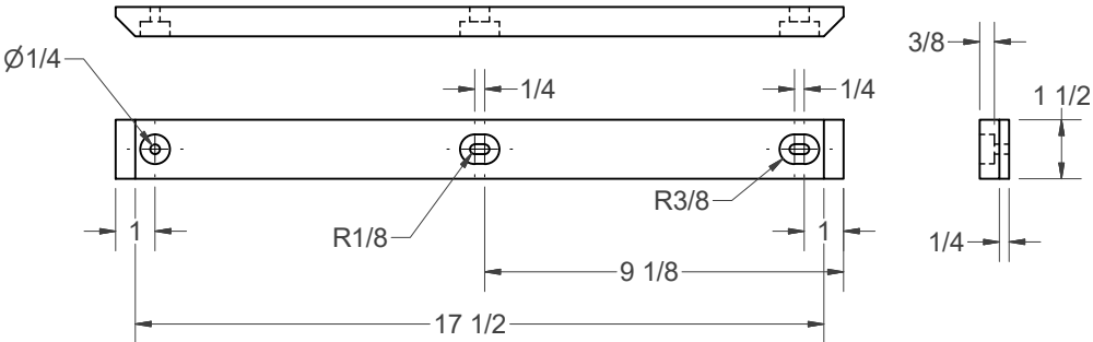
(BB) - MOUNTING CLEAT (2)
