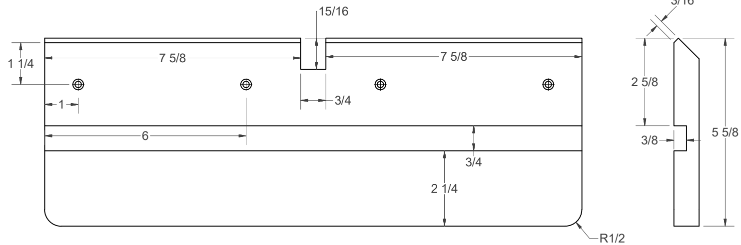
(A) - FRONT BED
