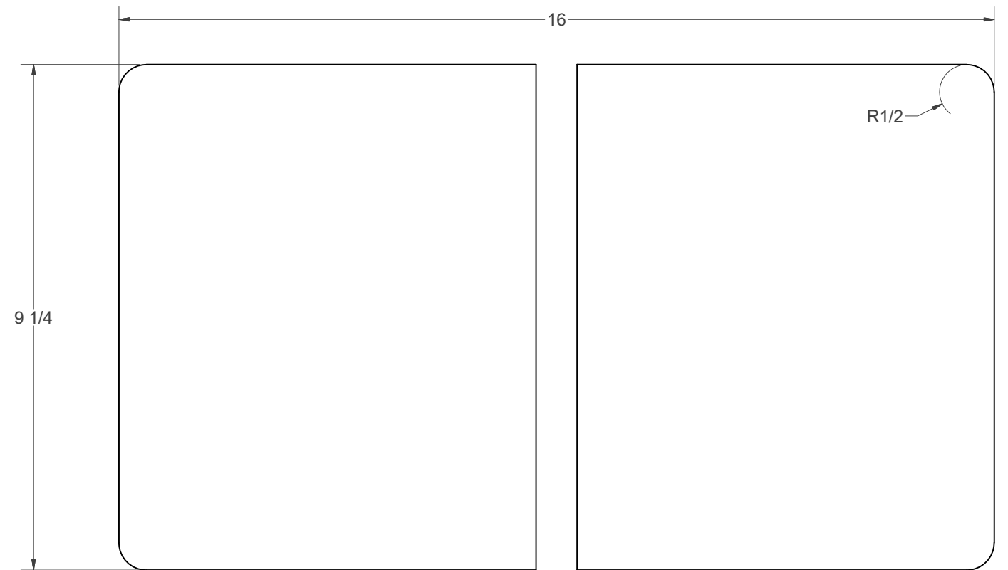
(E) - BASE
