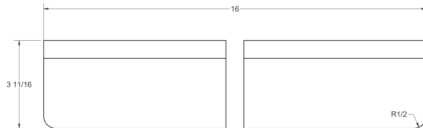
(C) - BED SUPPORT (QTY. 2)
