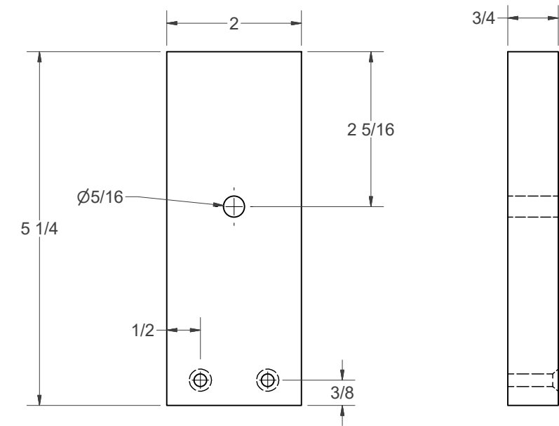
(G) - LONG STOP LEG (QTY. 2)
