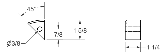
(E) - REAR GUIDE BLOCK
