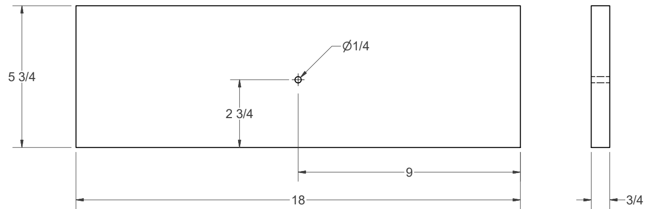
(A) - BASE
