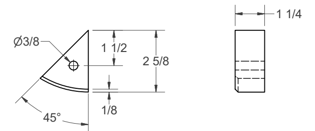
(F) - FRONT GUIDE BLOCK
