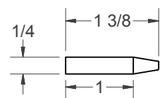
(O) - DRIVE PIN
