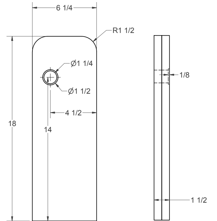
(E) - RIGHT SIDE
