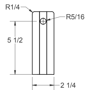
(P) - HEAD STOCK
