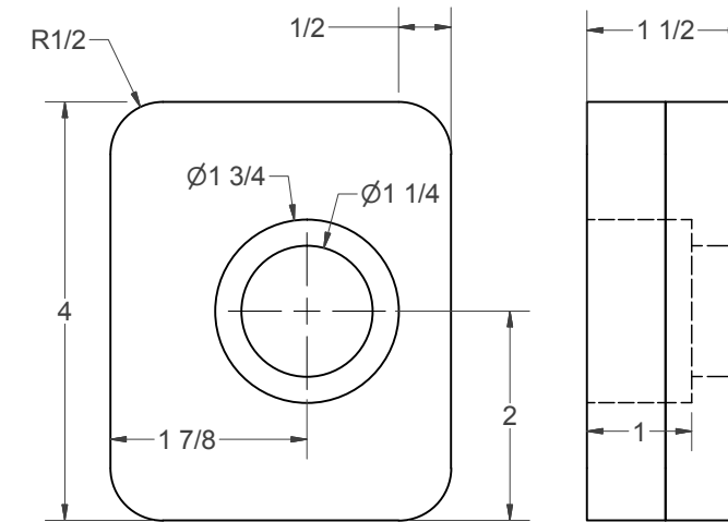
(LL) - TRAVELER BLOCK (NEED 2)
