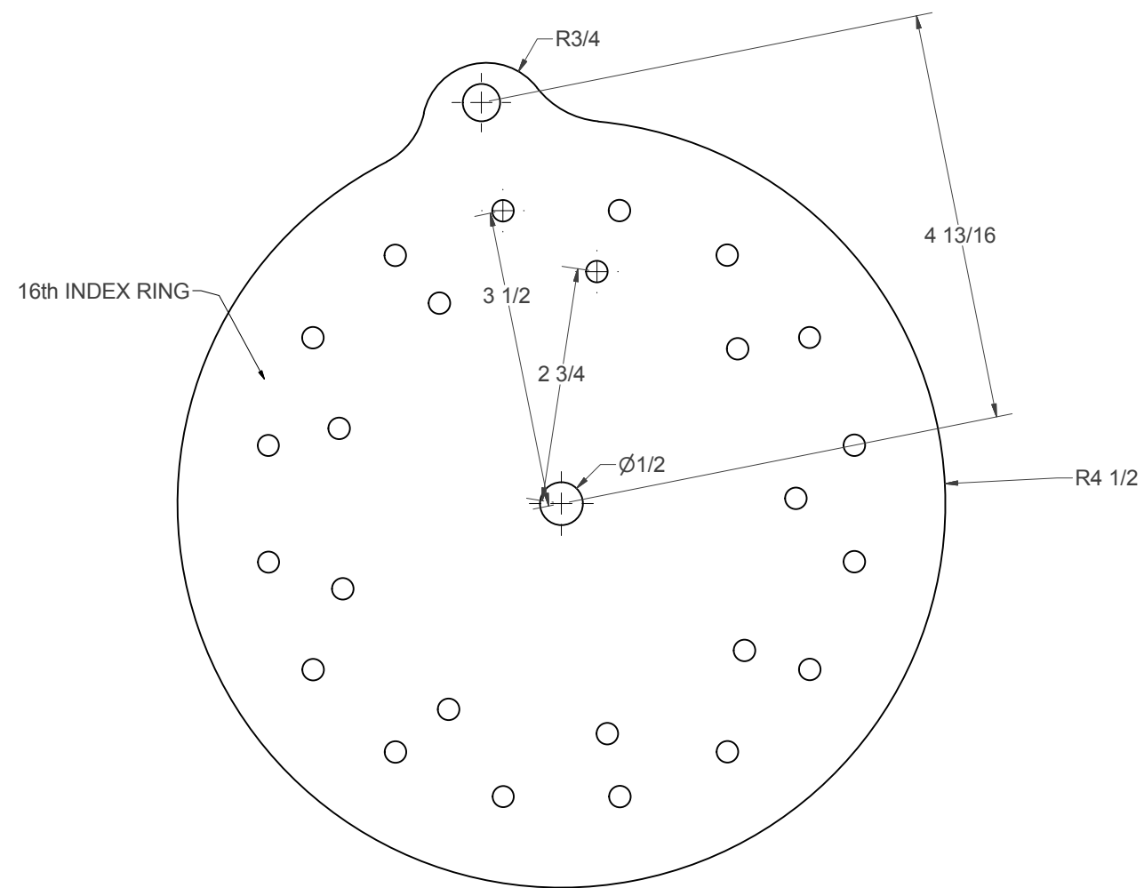
(U) - INDEXING WHEEL
