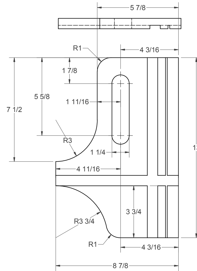
(HH) - LEFT SIDE
