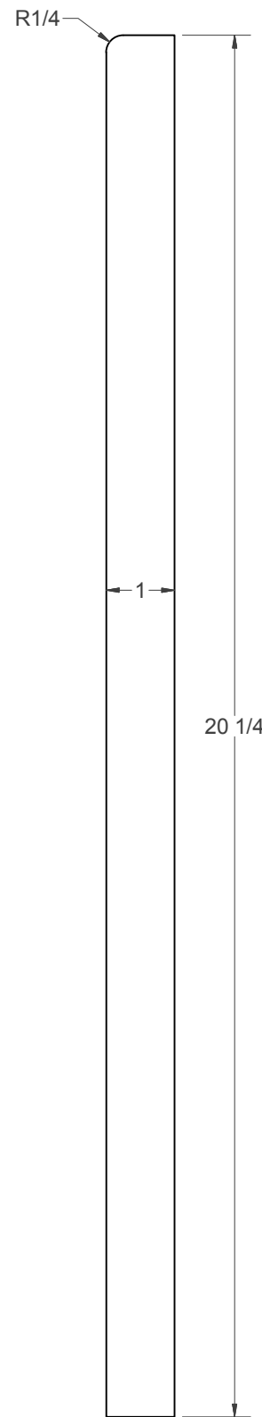
(DD) - GUIDE BAR (NEED 2)
