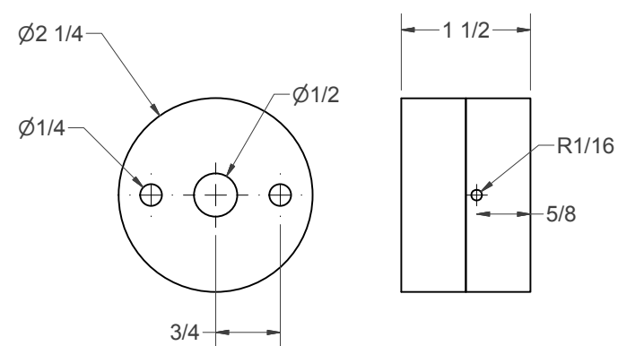
(W) - DRIVE DISK (NEED 2)
