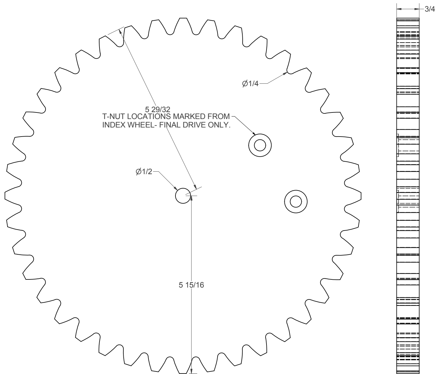
(AA) - 40 TOOTH GEAR
