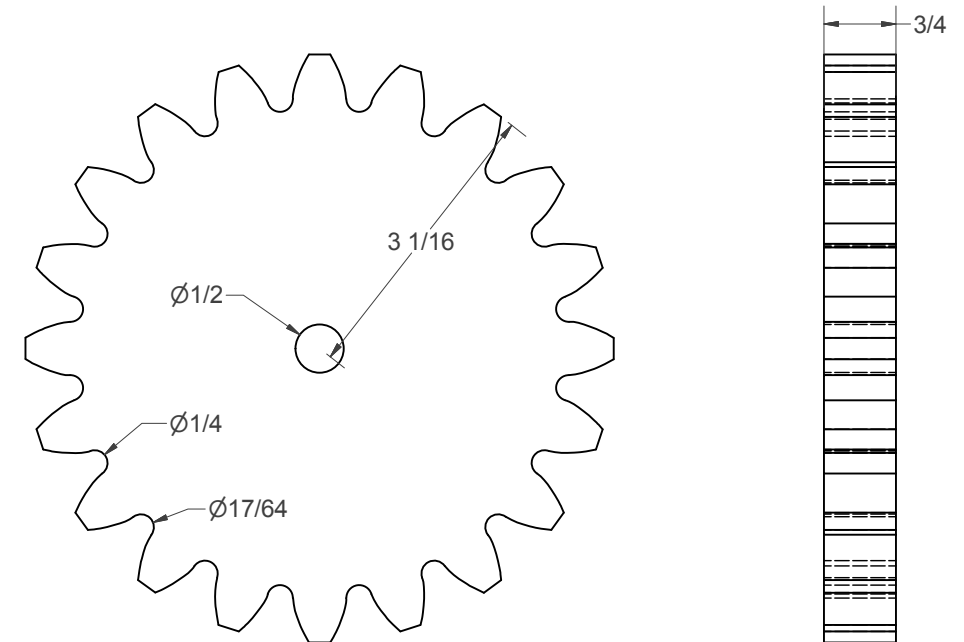
(Y) - 20 TOOTH GEAR
