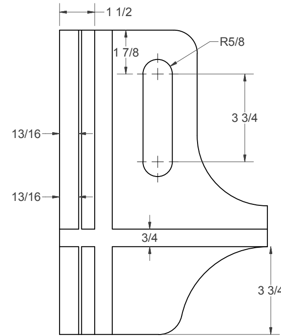
(HH) - RIGHT SIDE
