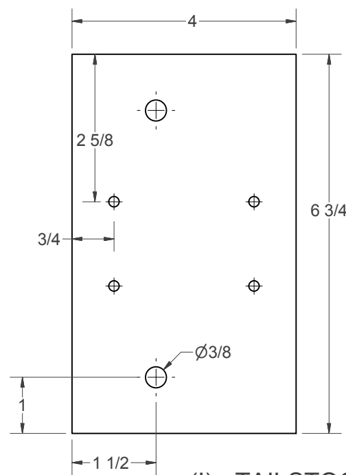
(I) - TAILSTOCK BASE
