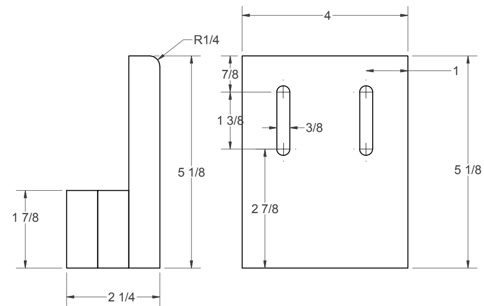
(L) - VERTICAL SUPPORT
