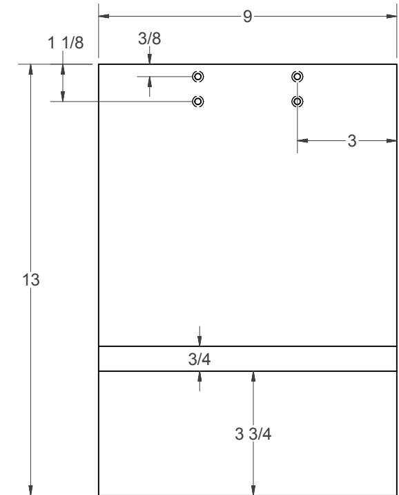
(II) - CARRIAGE BACK
