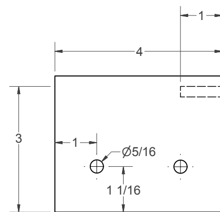
(N) - PIN BLOCK
