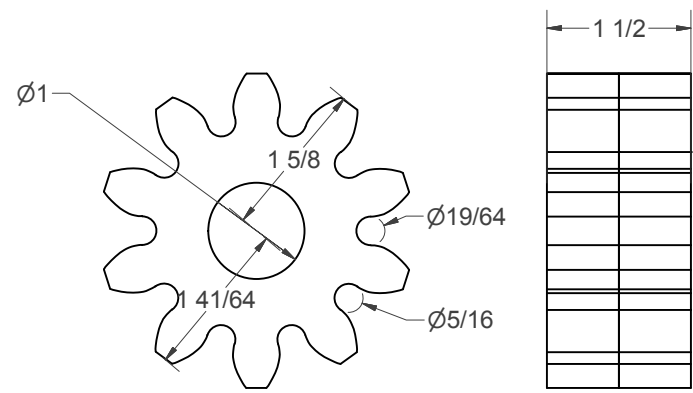
(R) - 10 TOOTH DRIVE GEAR (NEED 2)
