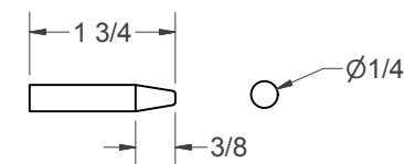
(O) - TAIL/DRIVE PINS
