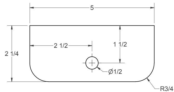
(EE) - LIFT BLOCK
