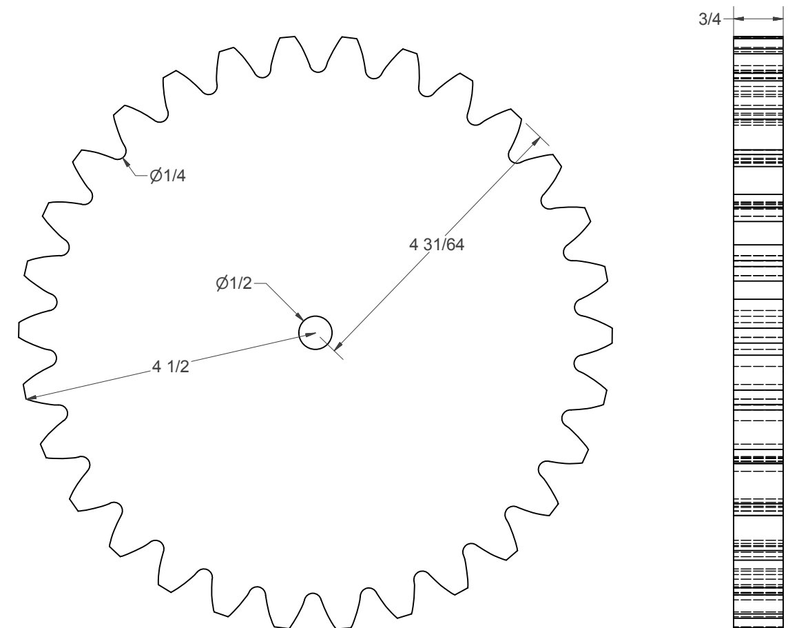
(Z) - 30 TOOTH GEAR
