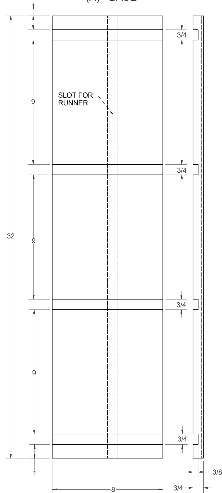
(A) - BASE
