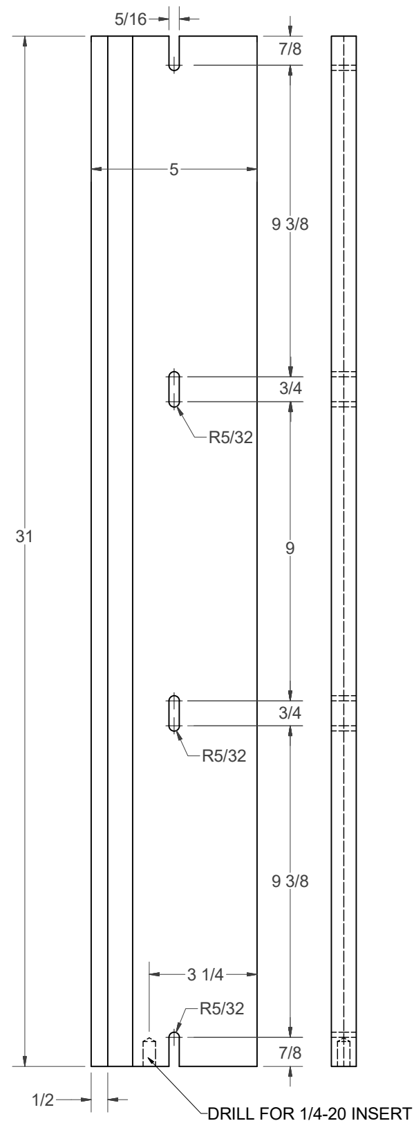
(C) - FENCE
