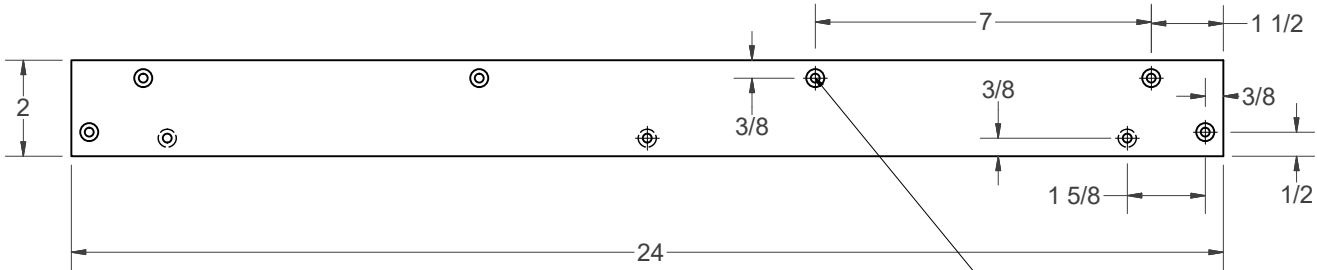
(F) - LONG MOUNTING STRIP (2)
