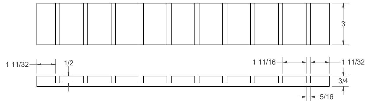
(I) - CLAMPS STRIPS (2)
