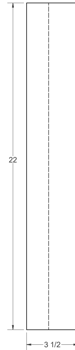
(A) - FRONT STILE (2)
