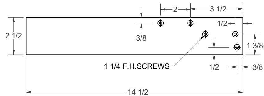
(J) - CLAMP RACK SIDE (2) ( MAKE MIRROR IMAGE )
