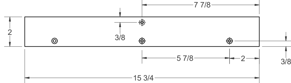
(G) - SHORT MOUNTING STRIP (2)
