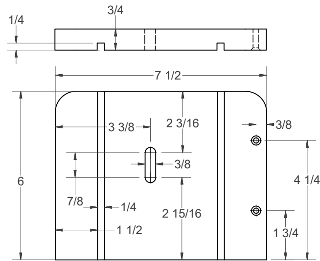
(H) - SUPPORT
