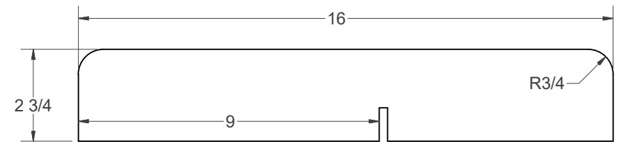
(B) - FRONT FENCE
