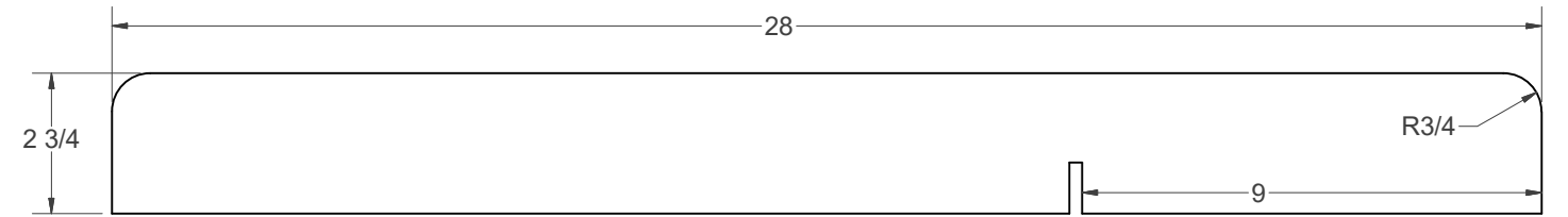
(C) - REAR FENCE
