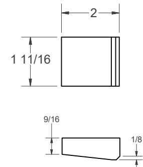
(M) - STOP
