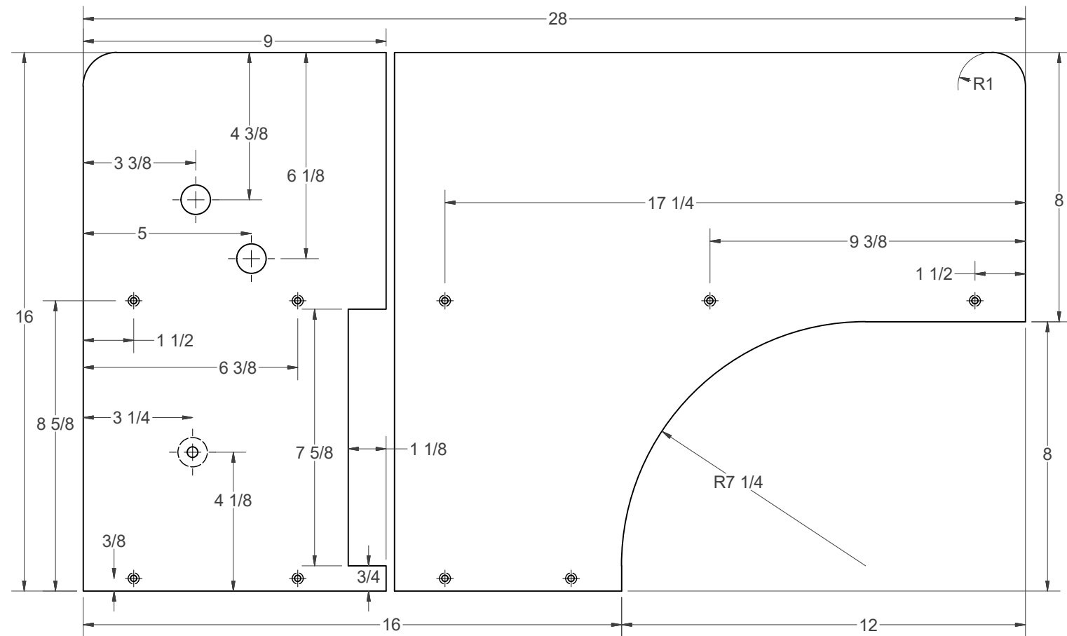
(A) - BASE
