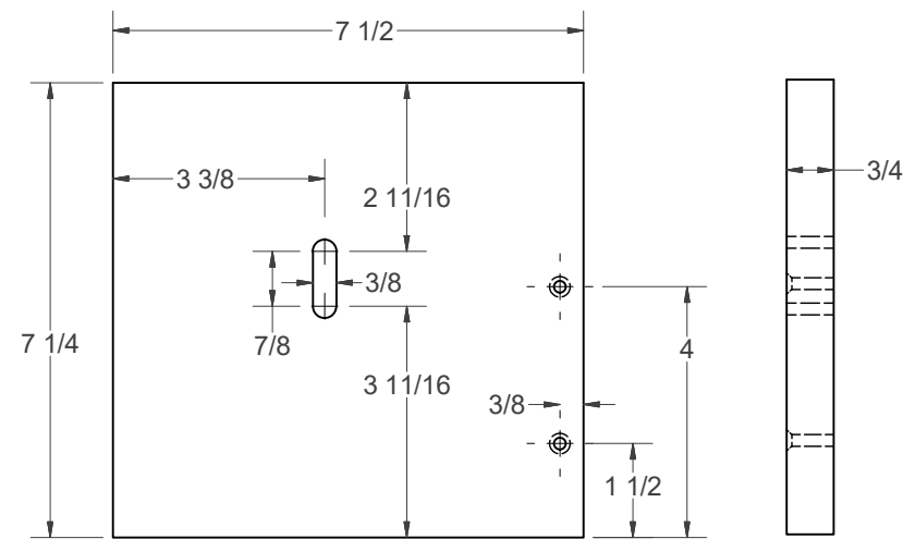
(F) - FENCE BASE
