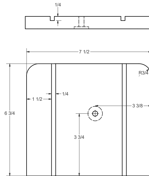
(G) - FENCE FACE
