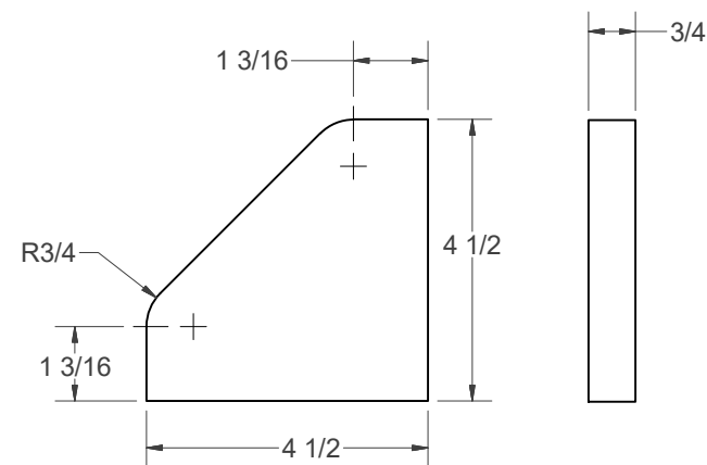
(I) - BRACE
