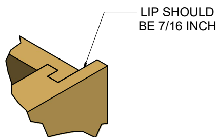
DETAIL J
