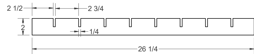
SHORT GRID STRIP ( 1/4\"/>
