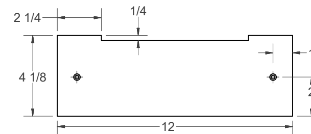
LIGHT SUPPORT 1/4" PLYWOOD
