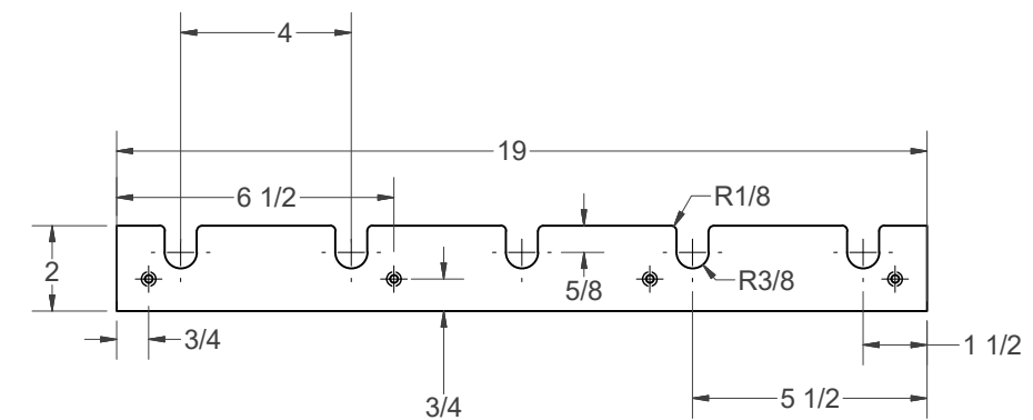
HANGER STRIP
