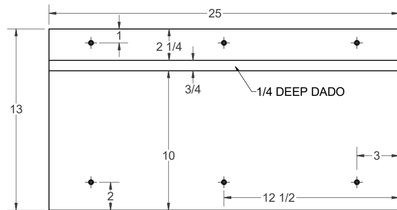
FRAME SIDE
