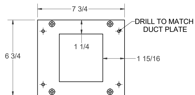
BLOWER FLANGE PLATE
