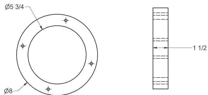
BLOWER STAND-OFF RING (2 PIECES 3/4" MDF)
