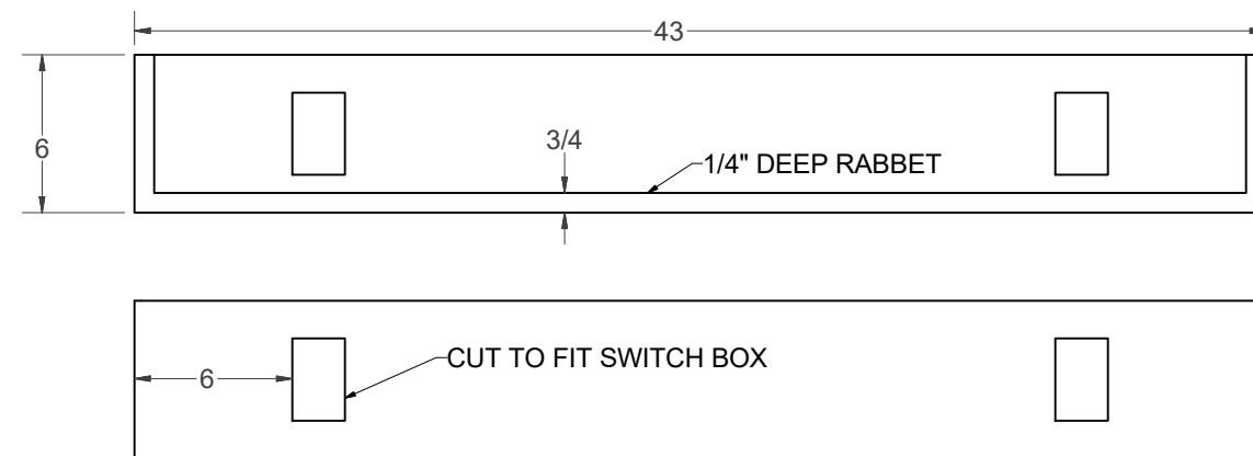
SWITCH PANEL
