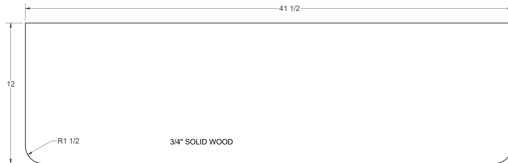
SHELF
