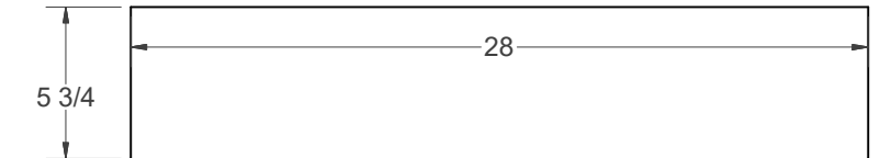
CASTOR PLATE
