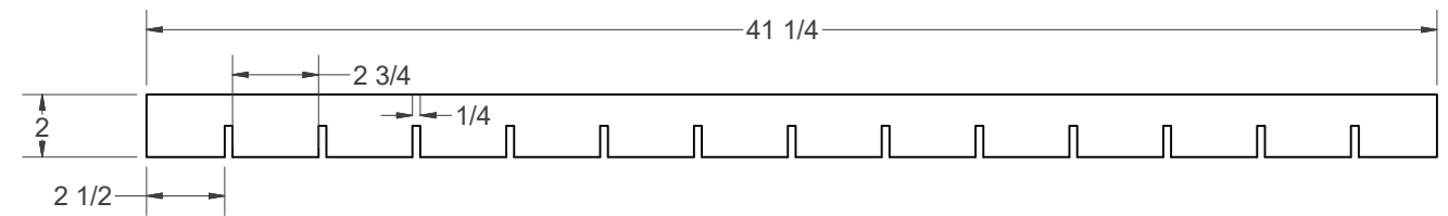
LONG GRID STRIP ( 1/4" PLYWOOD)
