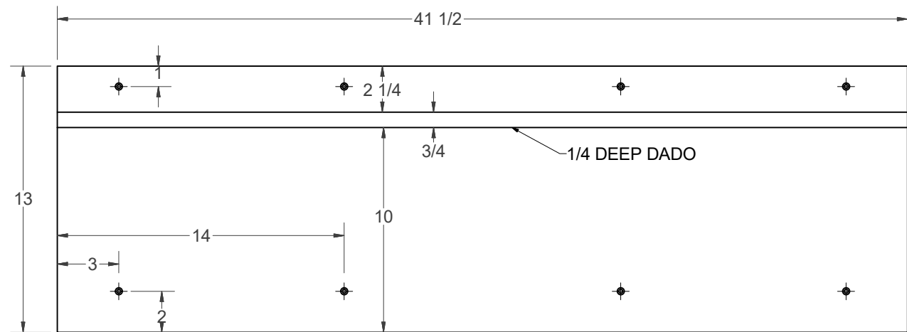
FRAME FRONT/BACK
