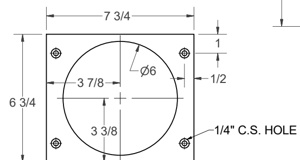
DUCT FLANGE PLATE
