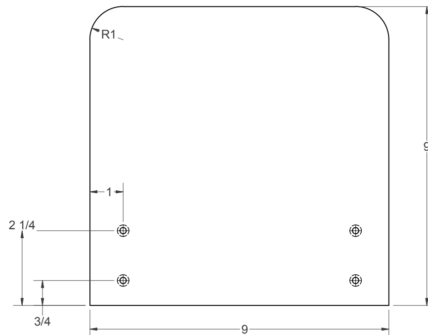
(I) - HOLDER END
