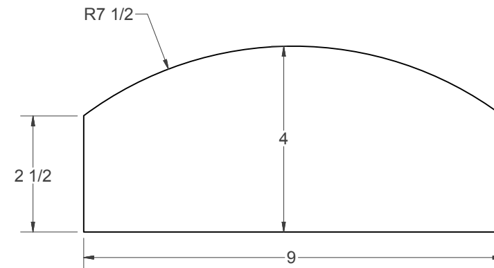
(H) - HOSE HOLDER (6 LAYERS 3/4" PLYWOOD)
