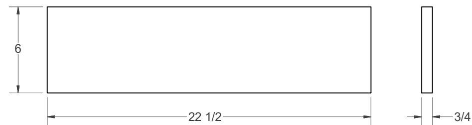
DRAWER FACE
