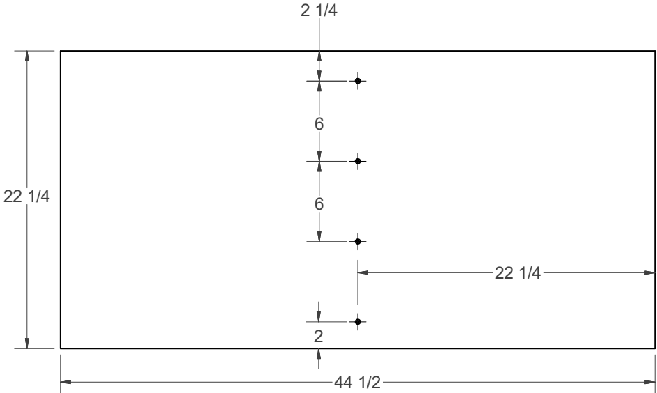
BENCH CLAMP SHELF
