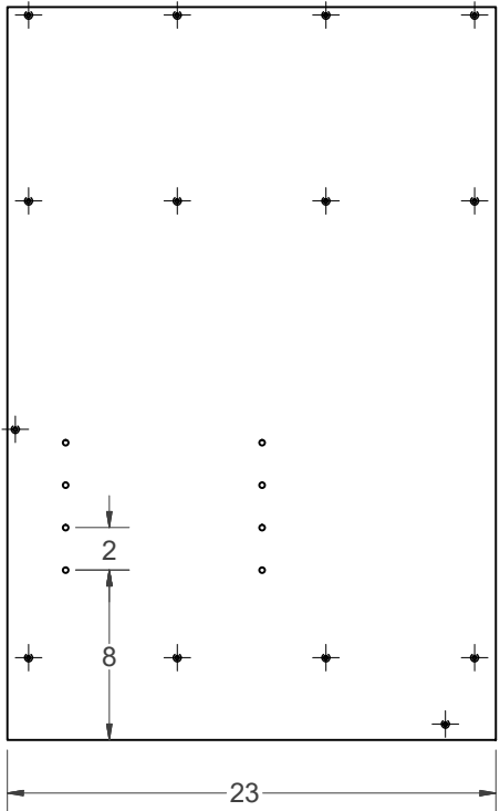
BENCH RIGHT SIDE (MIRROR OF LEFT SIDE)
