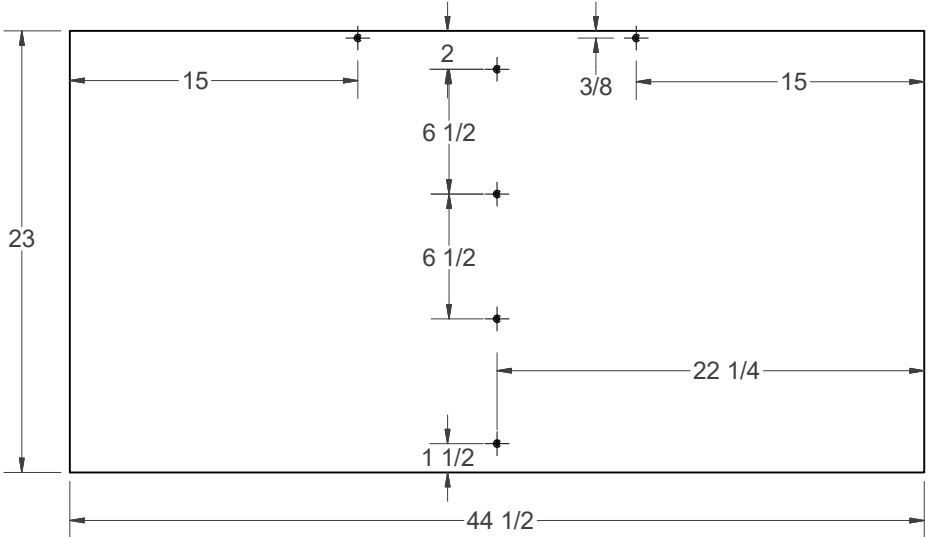
BENCH BASE PANEL
