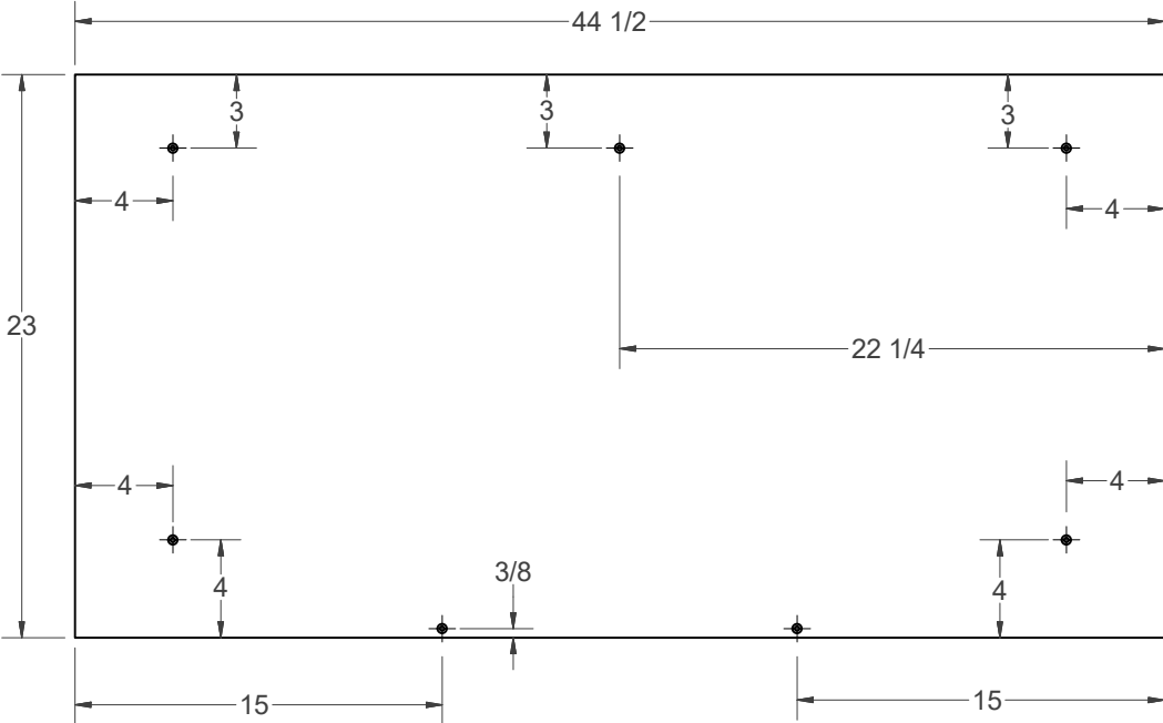
BENCH TOP PANEL
