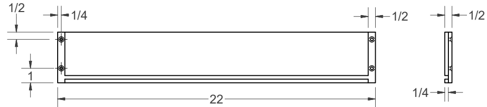
DRAWER SIDE
