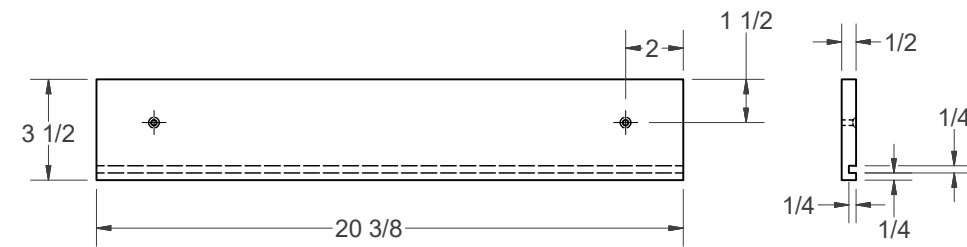
DRAWER BACK
