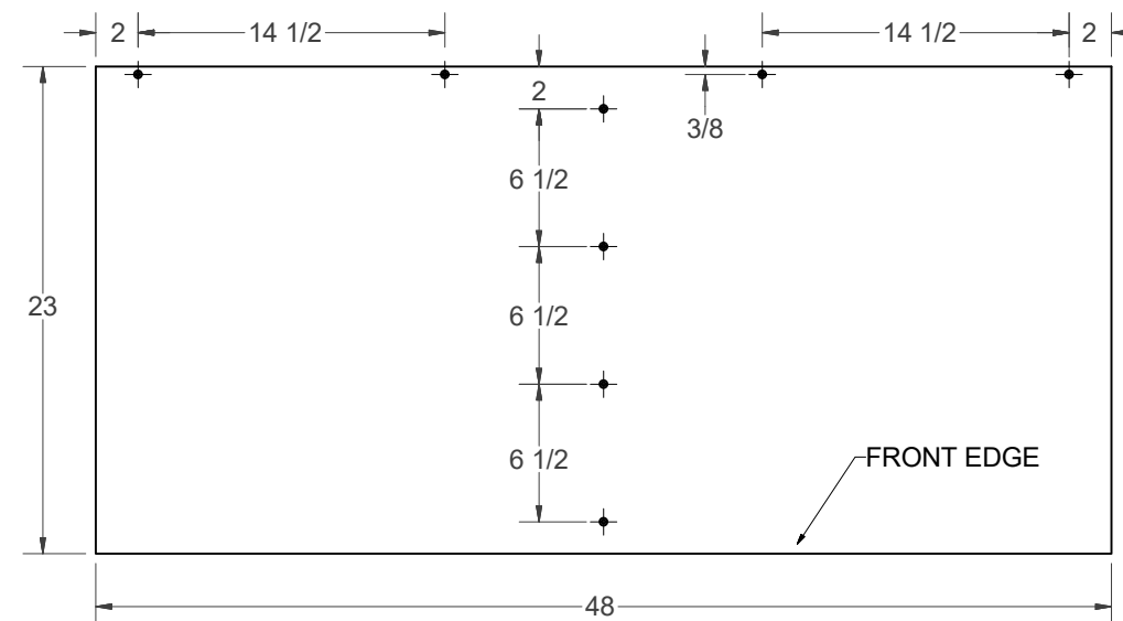
CENTER CAB. TOP/BOTTOM
