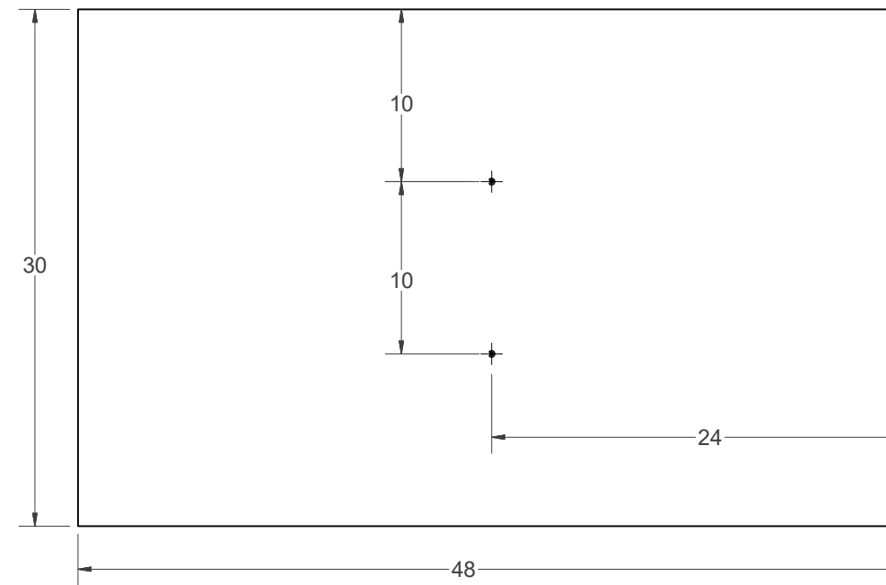
CENTER CAB. TOP/BOTTOM
