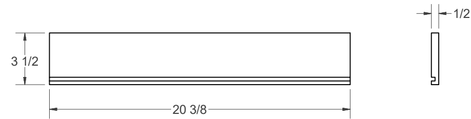
DRAWER SIDE
