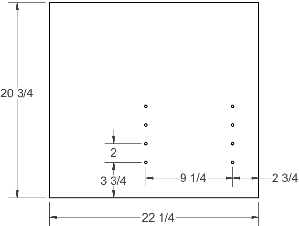
BENCH SHELF
