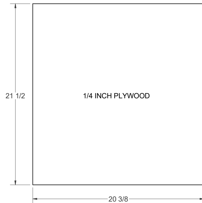
DRAWER BOTTOM
