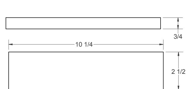
(Q) - ROUTER FENCE TOP (NEED 2)
