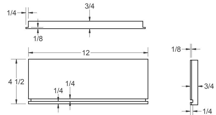
(J) - DRAWER BACK
