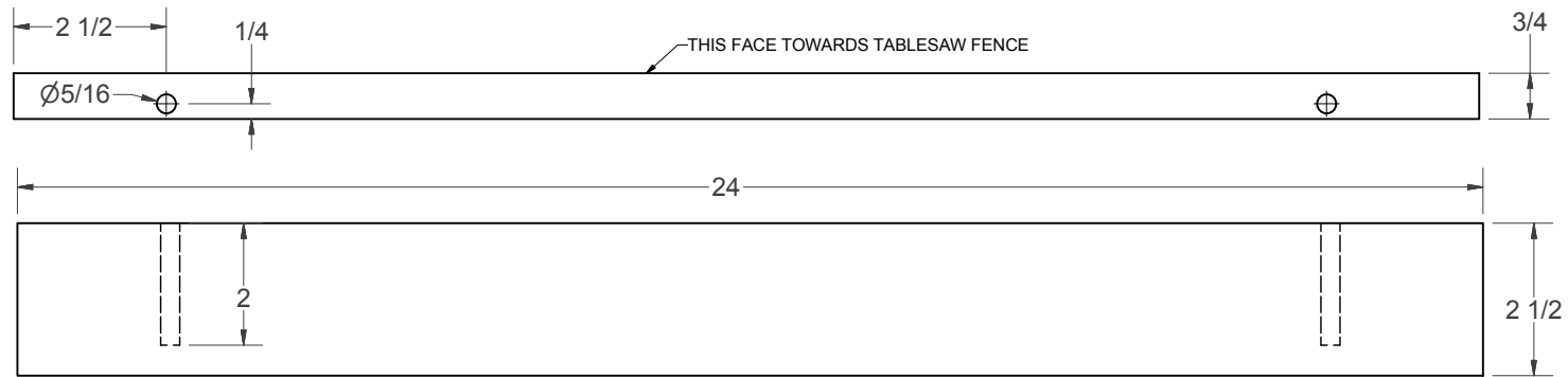
(P) - ROUTER FENCE BACK
