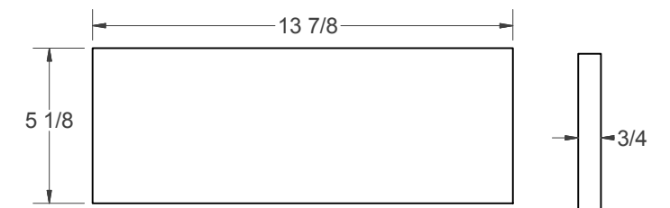
(L) - DRAWER FALSE FRONT
