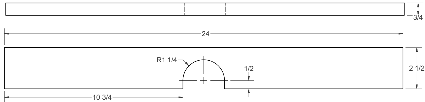
(P) - ROUTER FENCE FRONT
