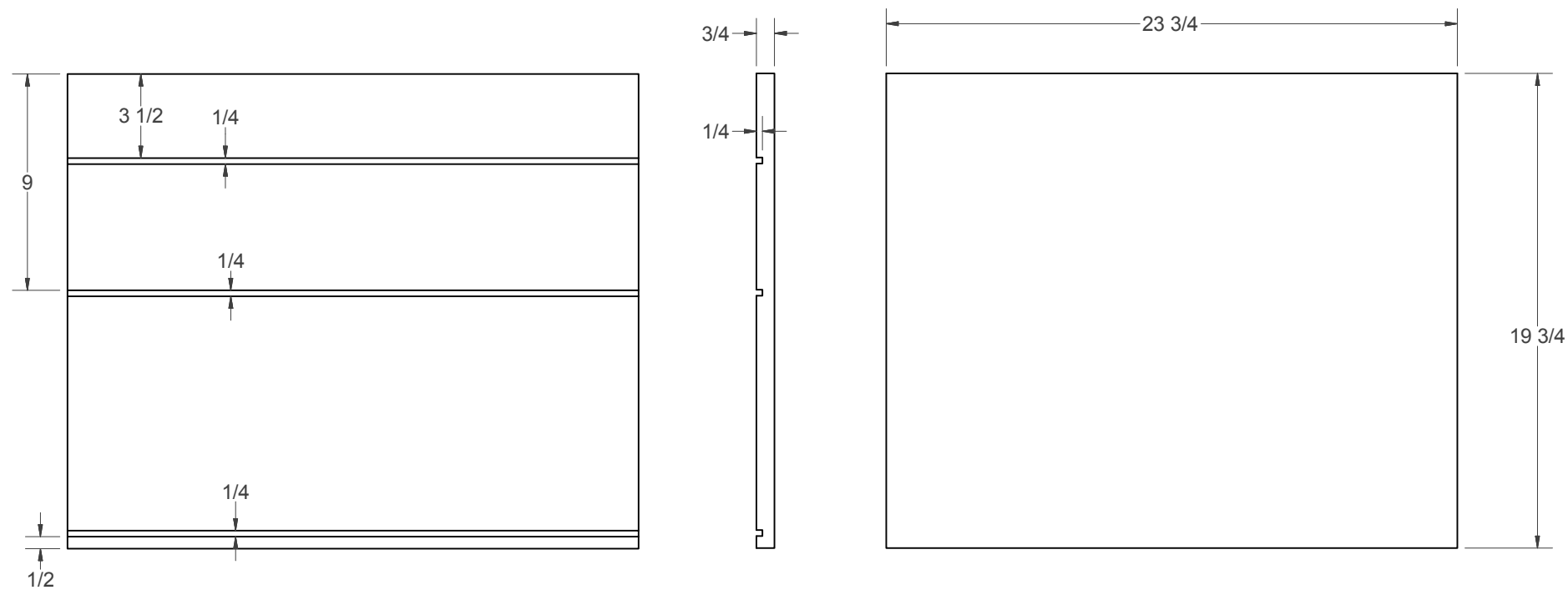
(F) - RIGHT SIDE
