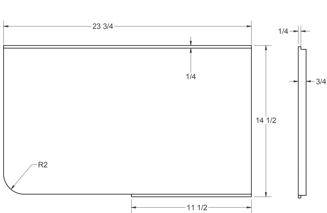
(G) - LOWER SHELF
