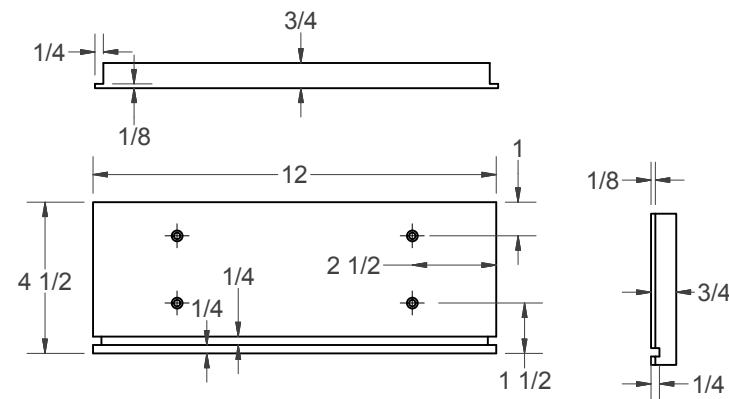
(J) - DRAWER FRONT
