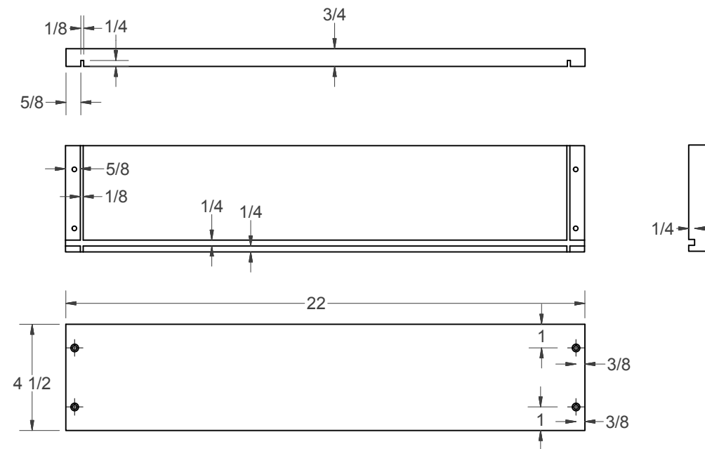
(I) - DRAWER SIDE (NEED 2)
