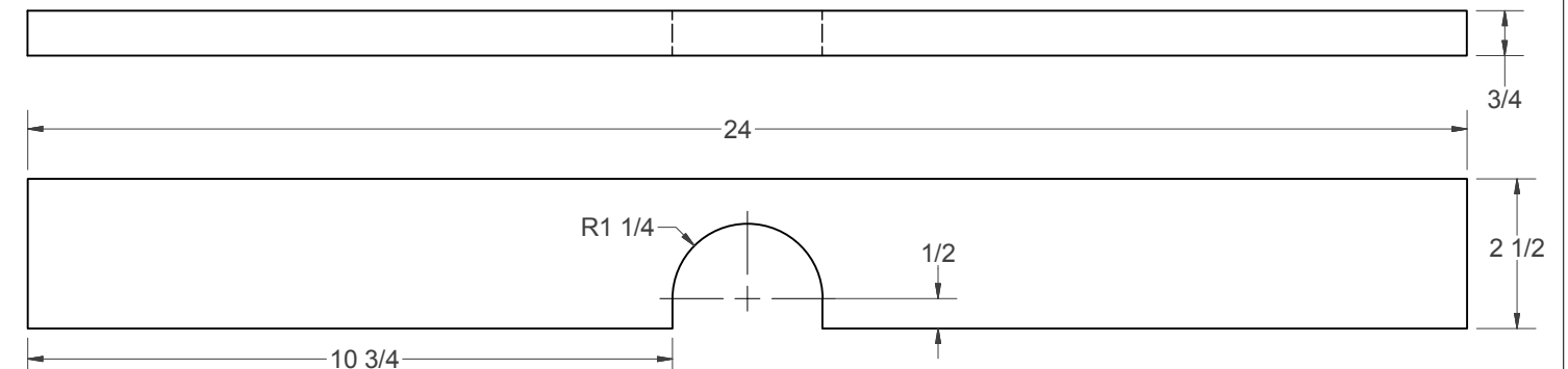
(P) - ROUTER FENCE BOTTOM
