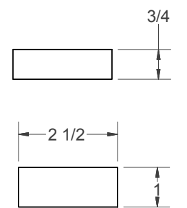
(R) - FILLER BLOCK (NEED 4)
