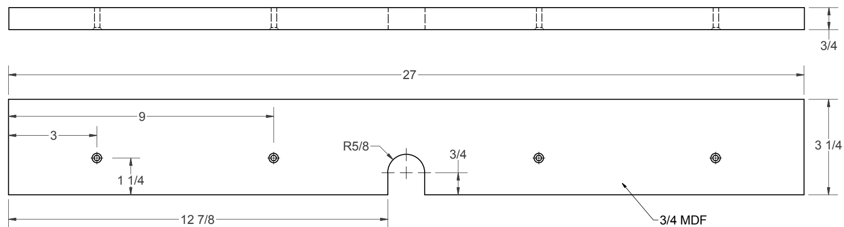
(S) - ROUTER FENCE FACE
