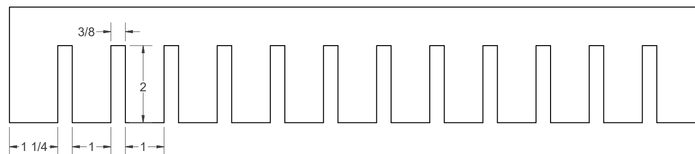
12 CLAMP RACK
