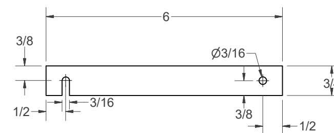
LATCH - 1/8" ALUMINUM
