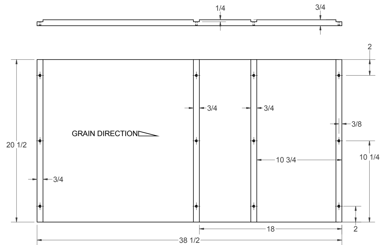
TOP AND BOTTOM
