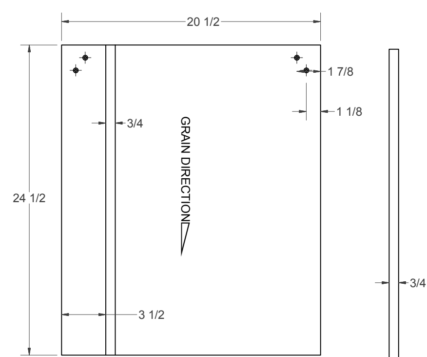
RIGHT END PANEL
