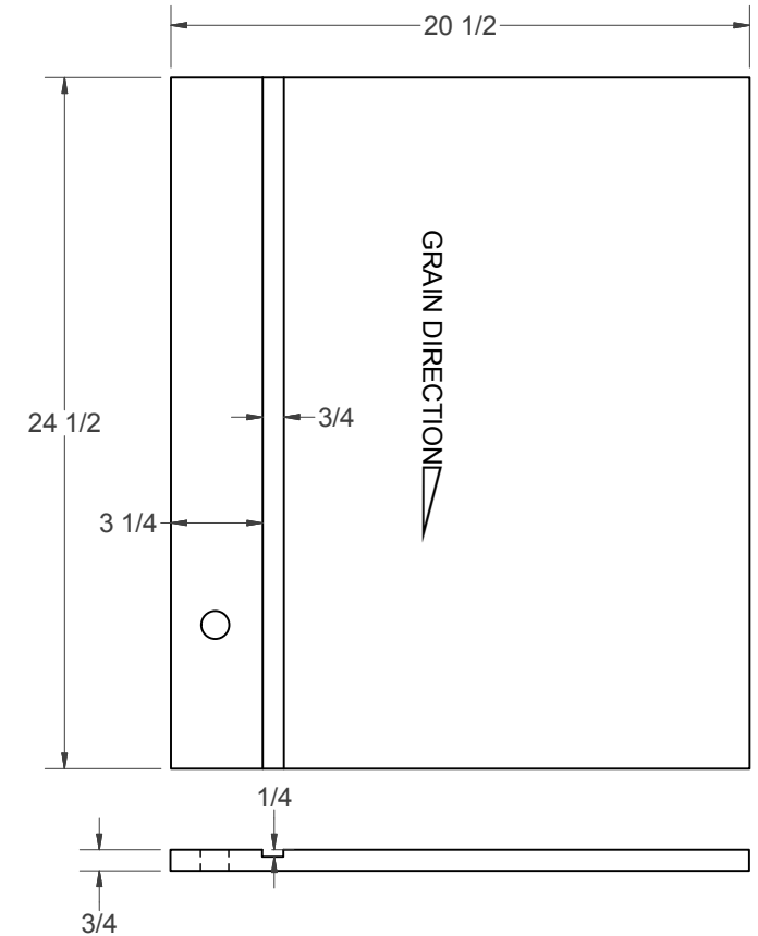
LEFT CENTER DIVIDER
