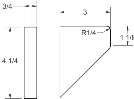
OUTER HANDLE BRACKET
