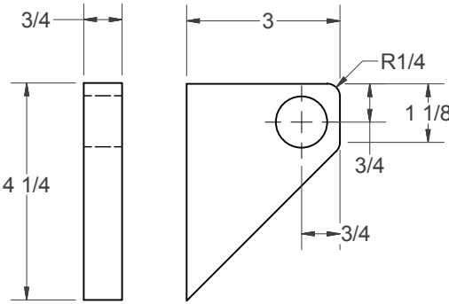
INNER HANDLE BRACKET
