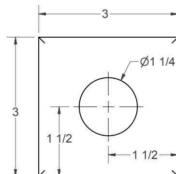
(K) - BASE VACUUM PORT (DRILL TO FIT HOSE)
