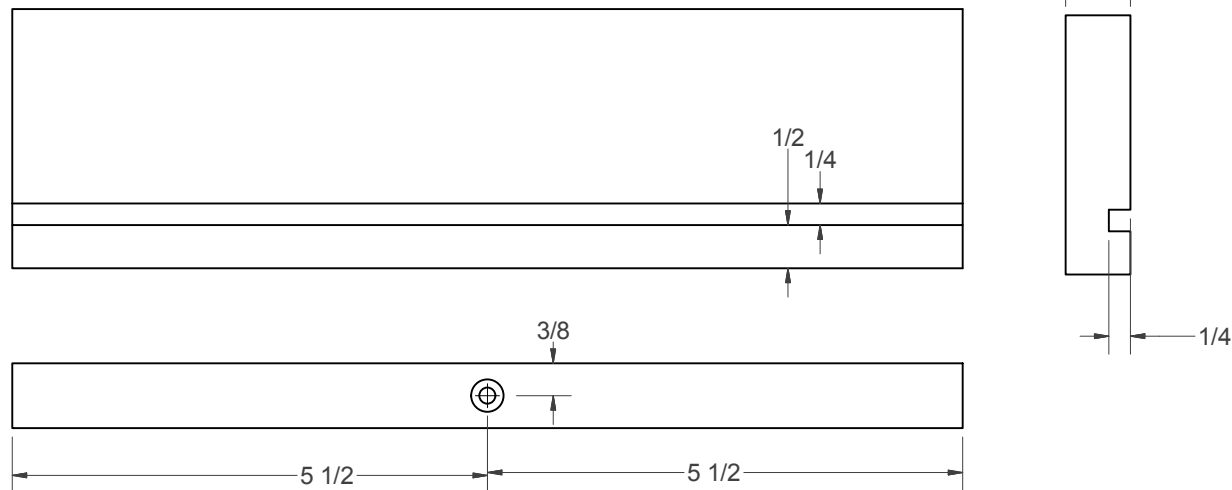
(G) - BASE BACK
