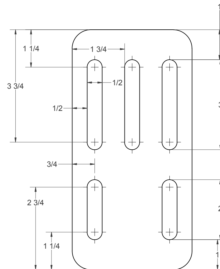
GENERAL USE VAC INSERT
