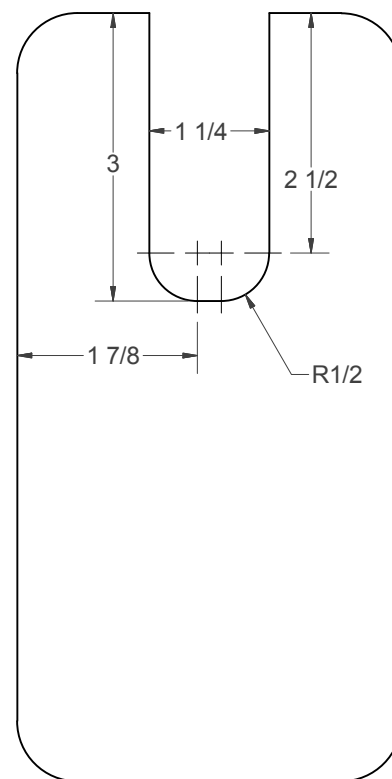
INSERT FOR FENCE
