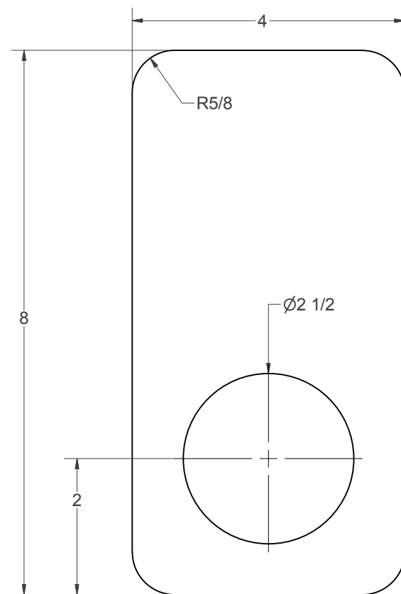
INSERT FOR DRUM SANDER
