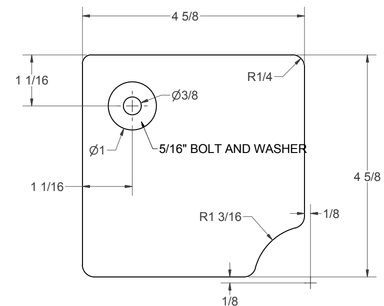
(C) - FILLER PLATE (4) (SHOWN FOR DELTA DRILL PRESS)
