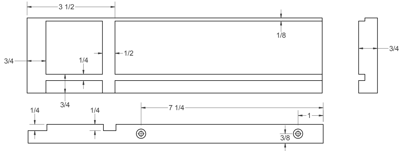
(F) - BASE SIDE (RIGHT)
