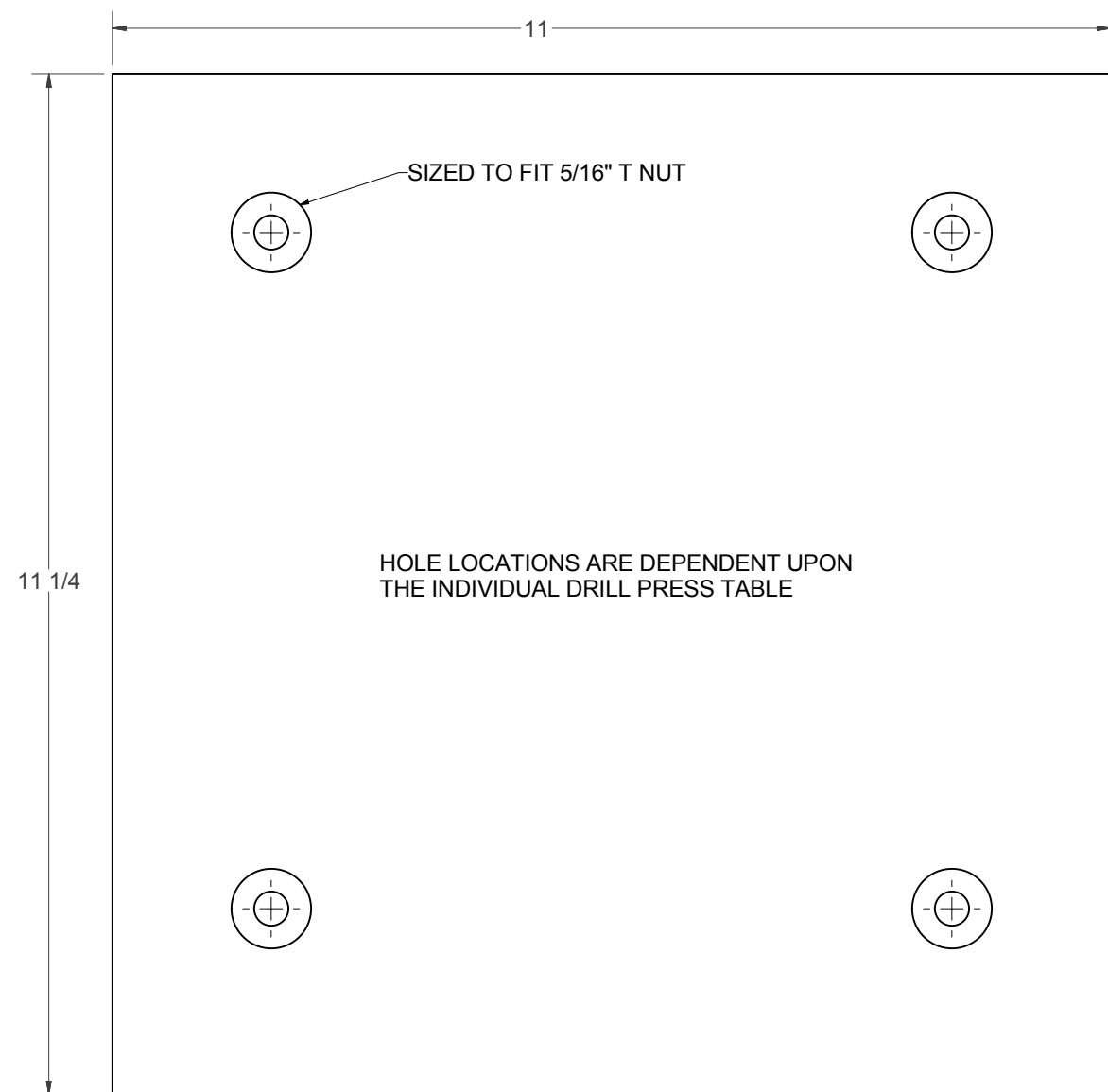
(I) - BASE BOTTOM
