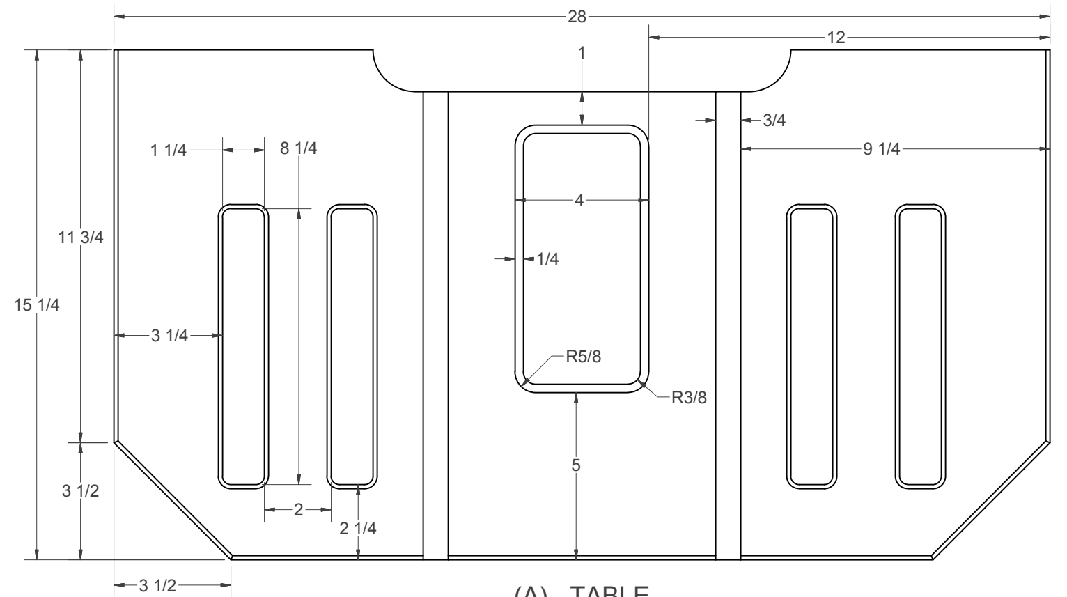
(A) - TABLE (TOP LAYER)
