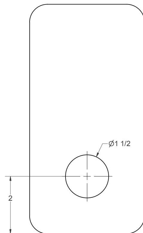
INSERT FOR DRUM SANDER
