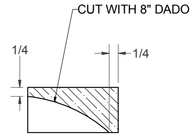
SECTION A-A SCALE 3 / 4
