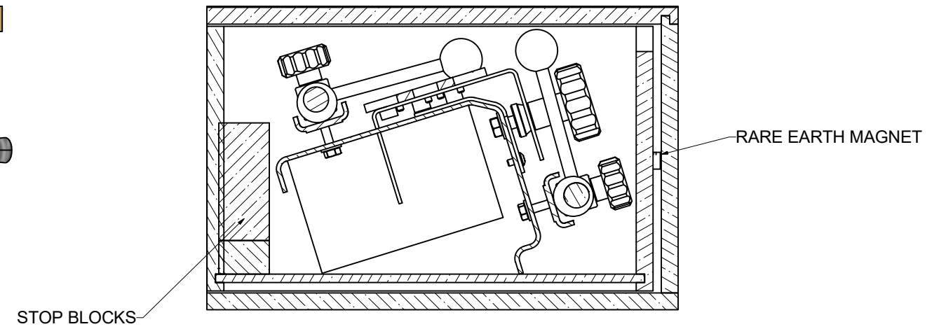
SECTION C-C SCALE 1 / 2
