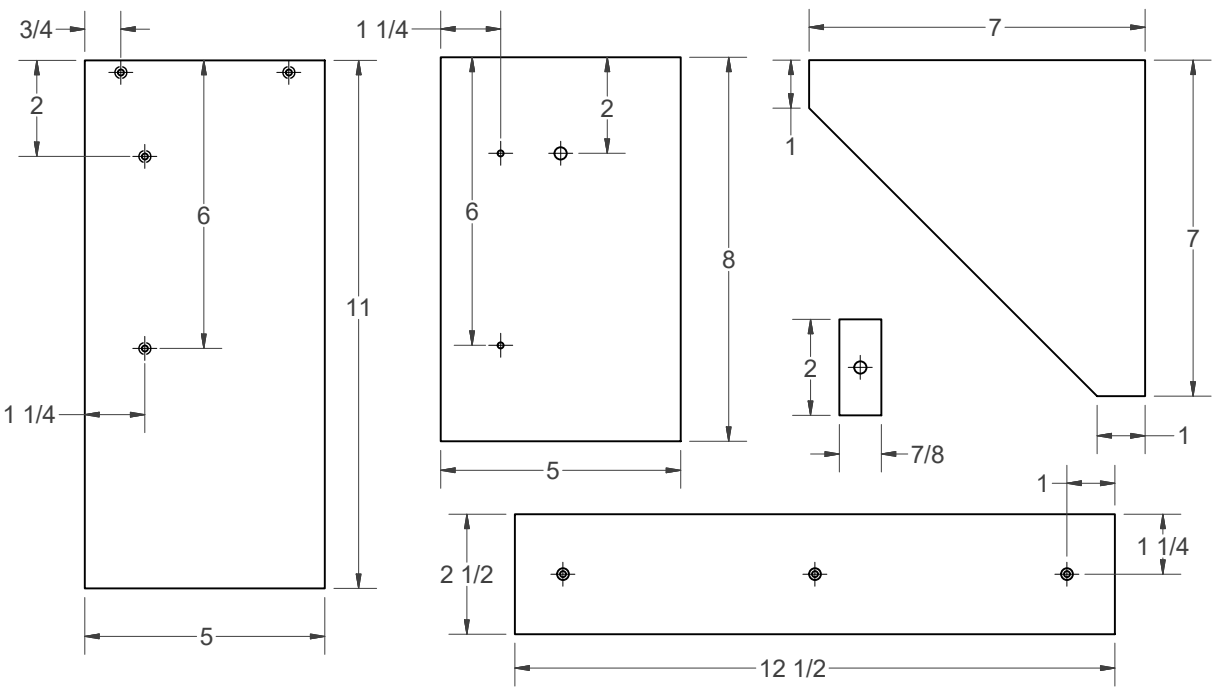
INFEED/OUTFEED PARTS
