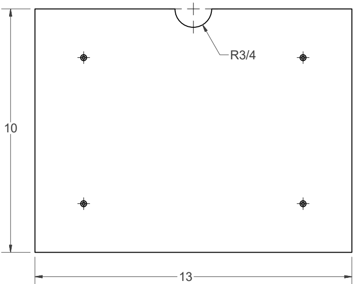
CASE BACK
