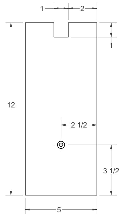
FILLER PLATE
