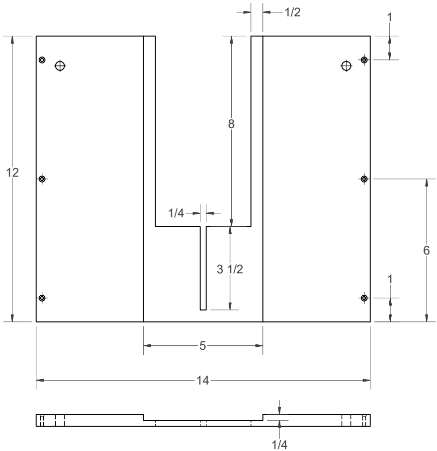
INFEED/OUTFEED PARTS
