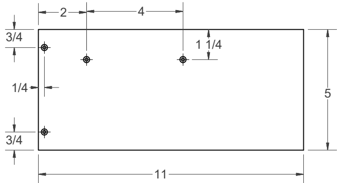
INFEED TOP
