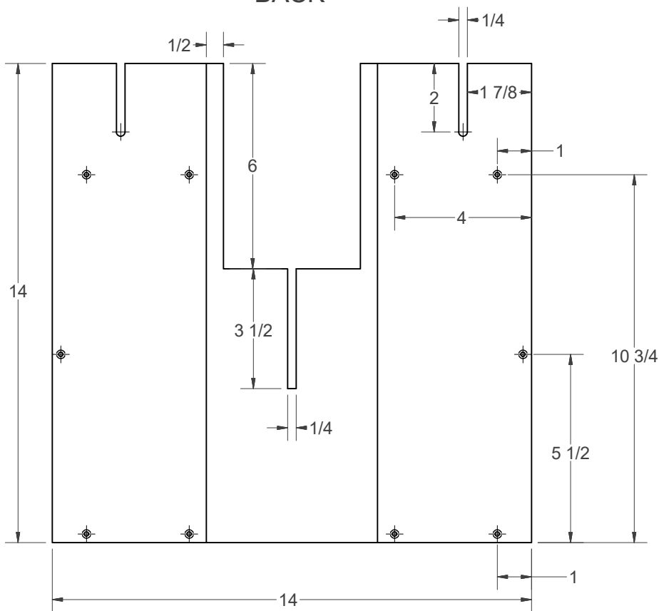
BACK
