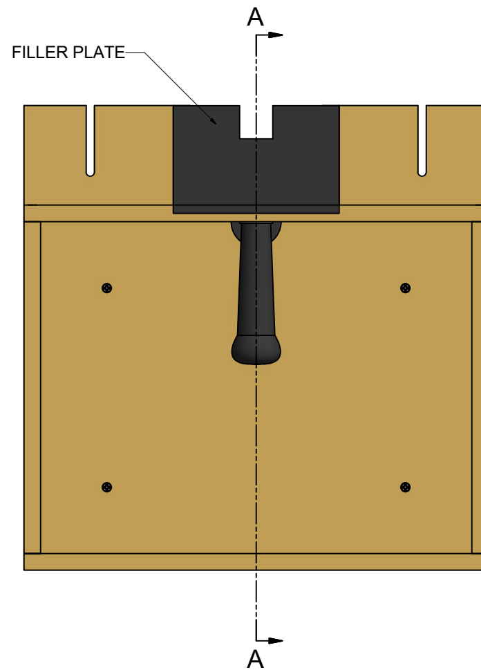
ROUTER PLATE
