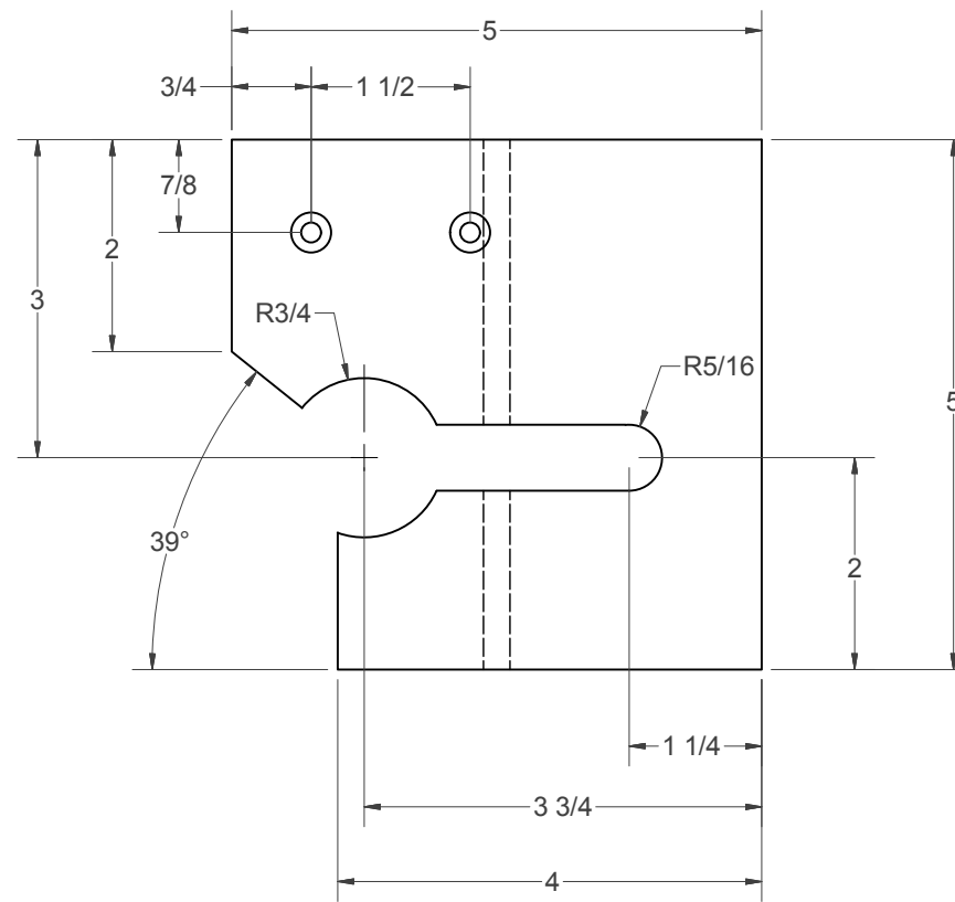
(K) - LOCK
