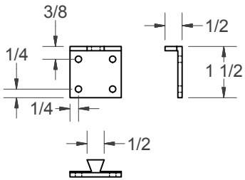
CABLE CATCH
