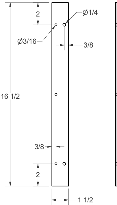
LOCK PLATE
