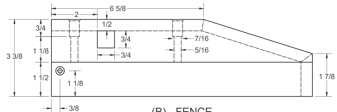
(B) - FENCE
