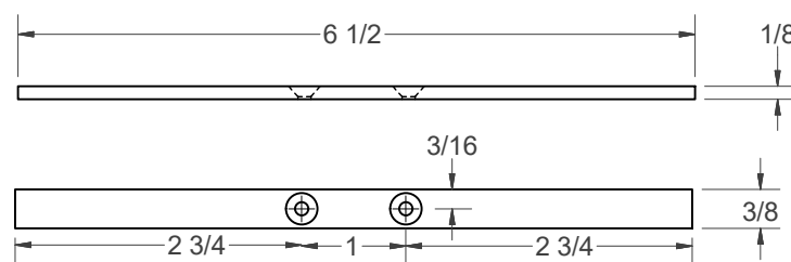
PRESSURE BAR
