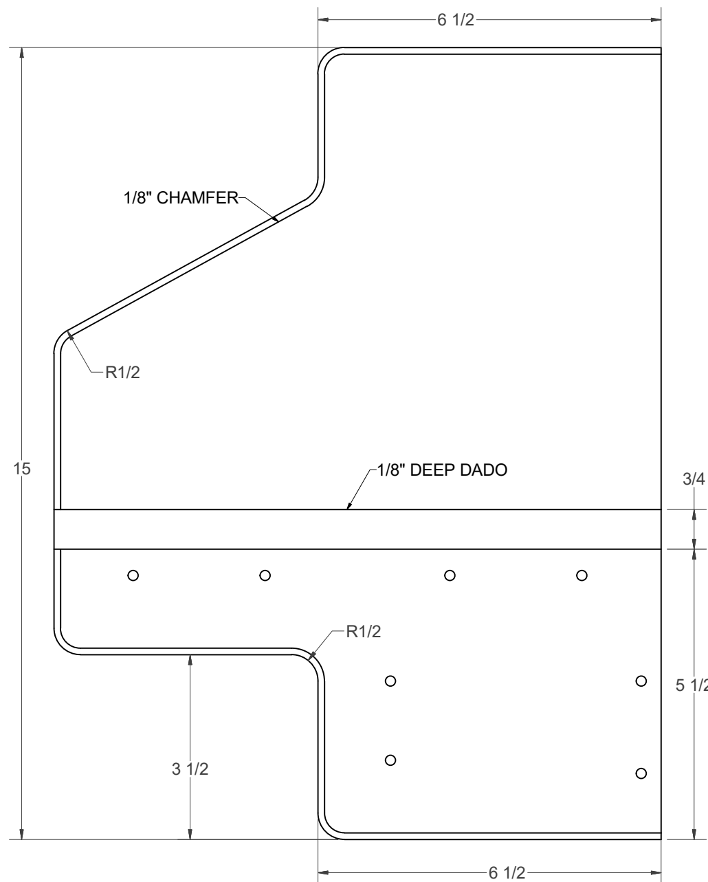
(A) - BASE
