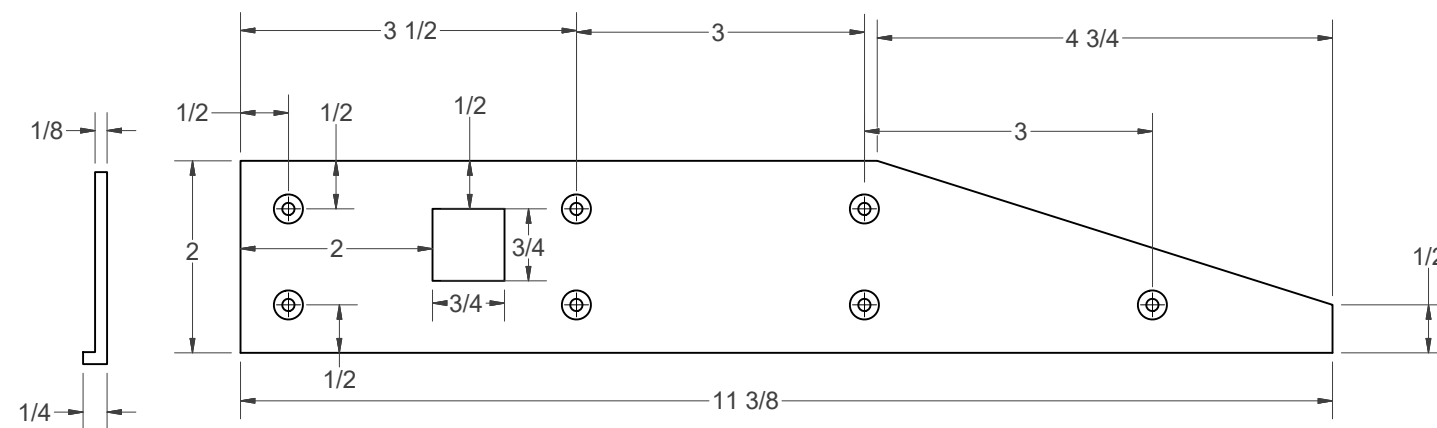
FENCE PLATE
