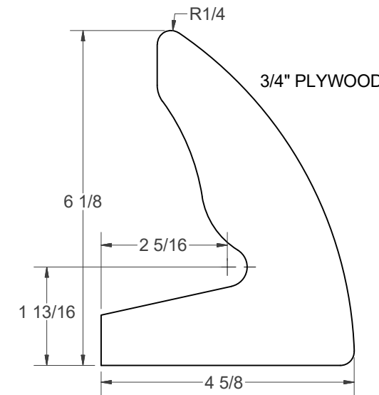
(F) - HANDLE
