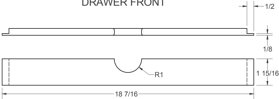
DRAWER FRONT
