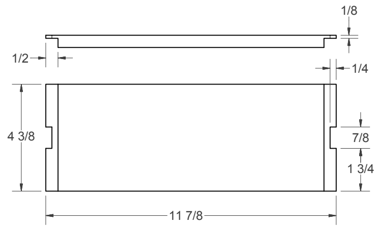
DRAWER BACK
