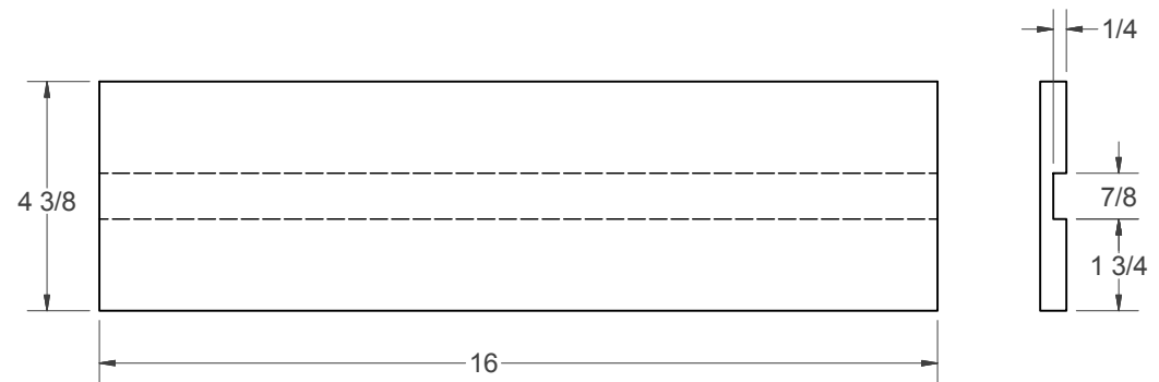
DRAWER SIDE
