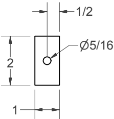
PINCH BLOCK
