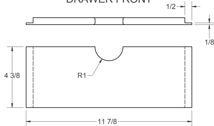
DRAWER FRONT
