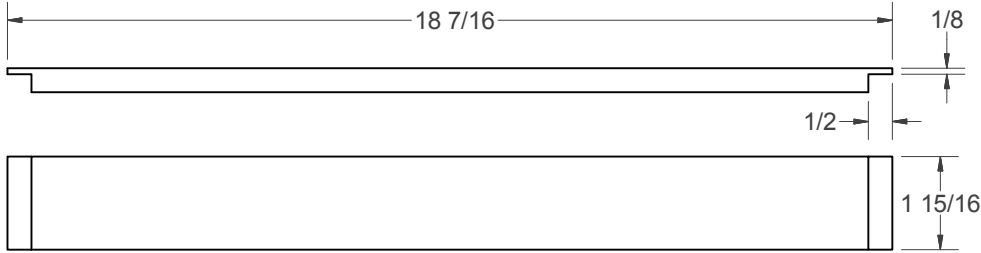
DRAWER BACK
