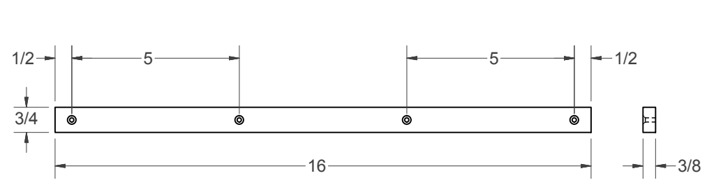
DRAWER GUIDE
