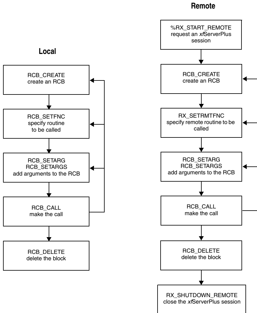
Figure 15-1. Making local and remote calls using a routine call block.
