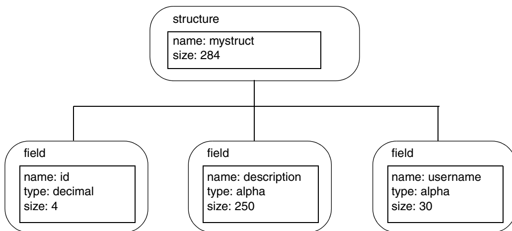
Figure 18-1. A DOM tree of an XML document.
