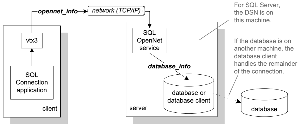
Figure 2-1. Using SQL OpenNet to connect to a database or database client.
