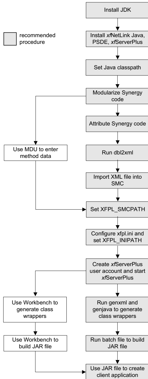
Figure 7-2. Steps in creating an xfNetLink Java – xfServerPlus application.
