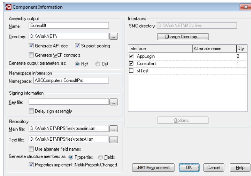
Figure 10-3. The Component Information dialog box for a Synergy/DE .NET Component project.
