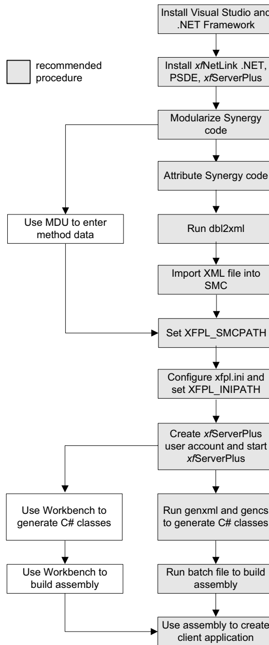
Figure 10-2. Steps in creating an xfNetLink .NET – xfServerPlus application.
