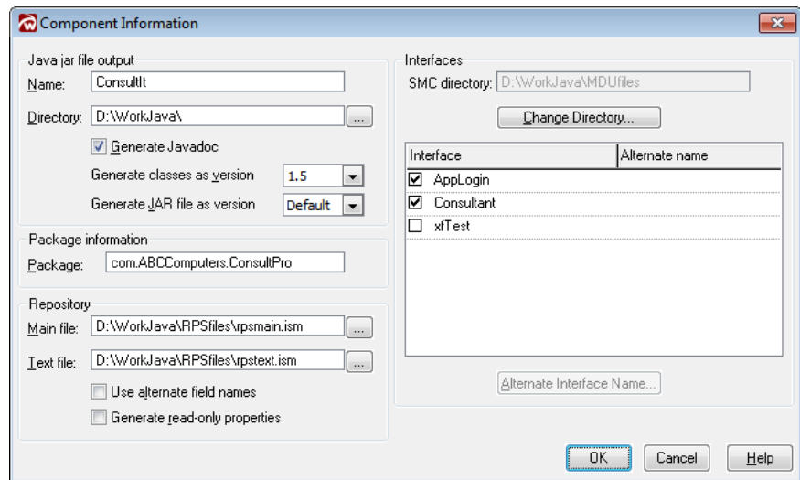
Figure 7-3. The Component Information dialog box for a Synergy/DE Java Component project.
