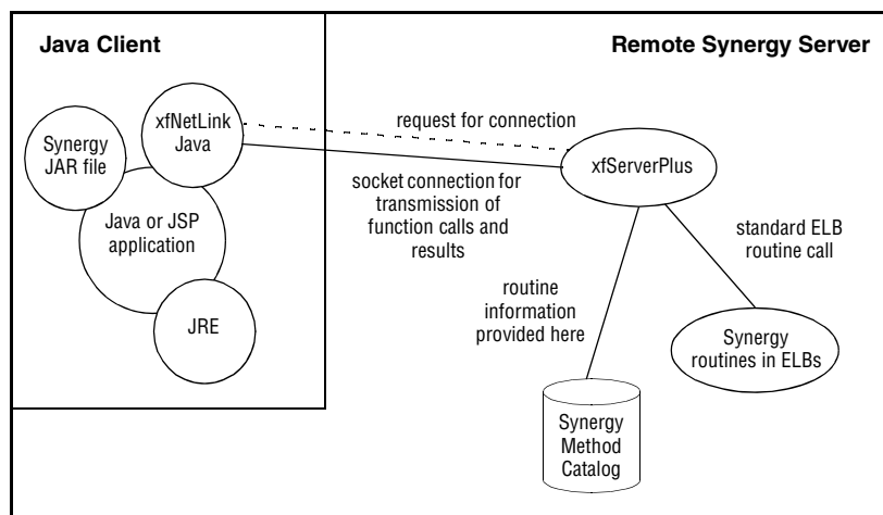
Figure 7-1. Accessing Synergy from Java.
