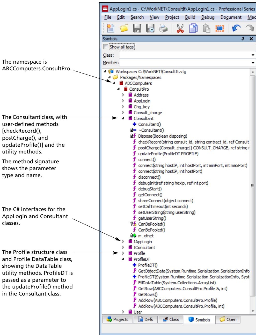
Figure 10-4. Viewing the generated C# classes and C# interfaces in Workbench.
