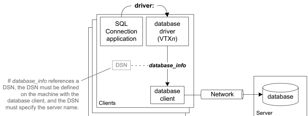
Figure 2-3. Connecting directly to a remote database (via a local database client).
