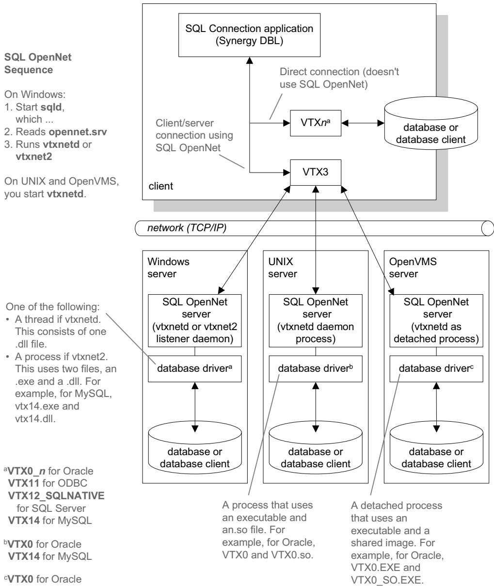
Figure 1-2. SQL OpenNet connections and direct connections (client/server and stand-alone).
