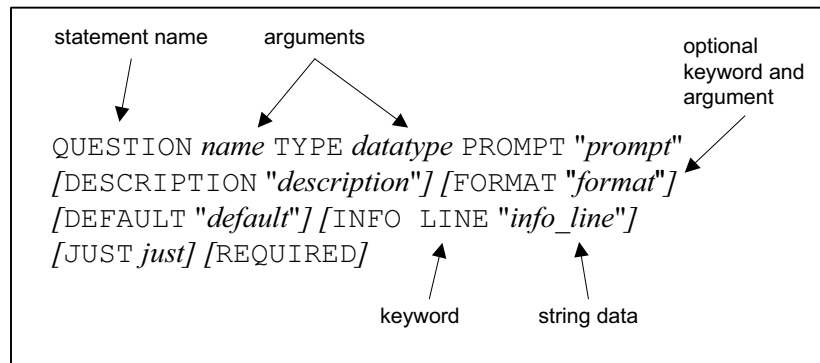
Figure 17-1. Report Definition Language syntax
