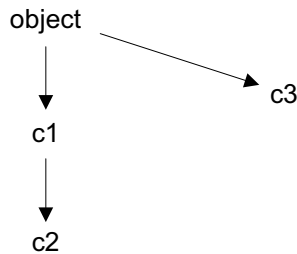
Figure 8-1. Class hierarchy.
