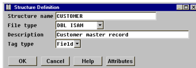
Figure 2-2. Defining a structure.
