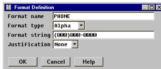
Figure 3-9. Defining a format.
