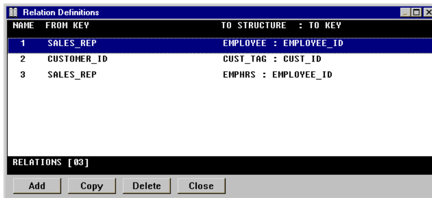
Figure 4-5. The Relation Definitions list.
