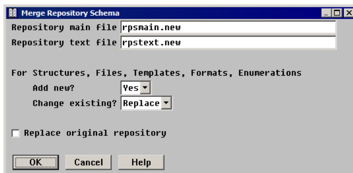
Figure 5-7. Merging a repository schema.
