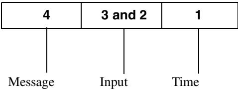
Figure 9-7. %WAIT parameters.
