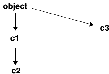
Figure 8-1. Class hierarchy.
