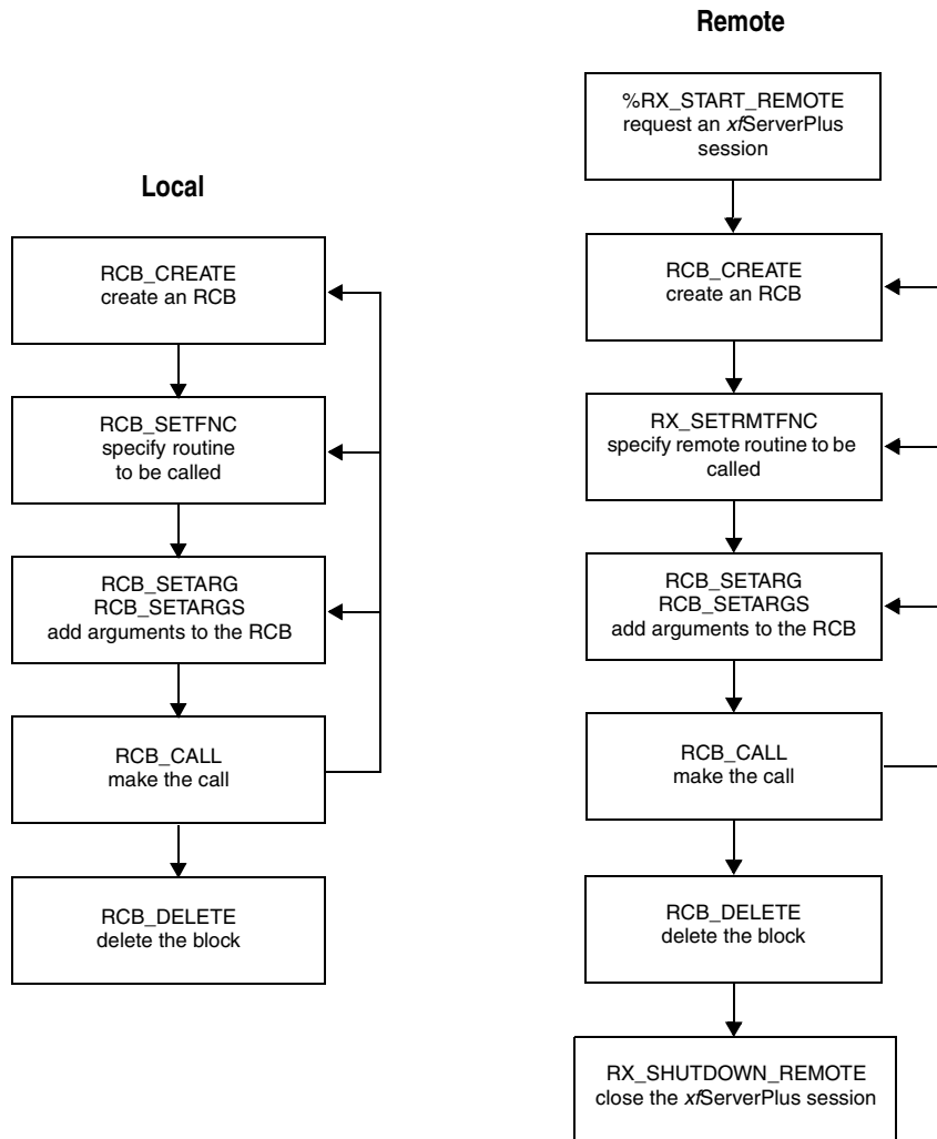
Figure 16-1. Making local and remote calls using a routine call block.
