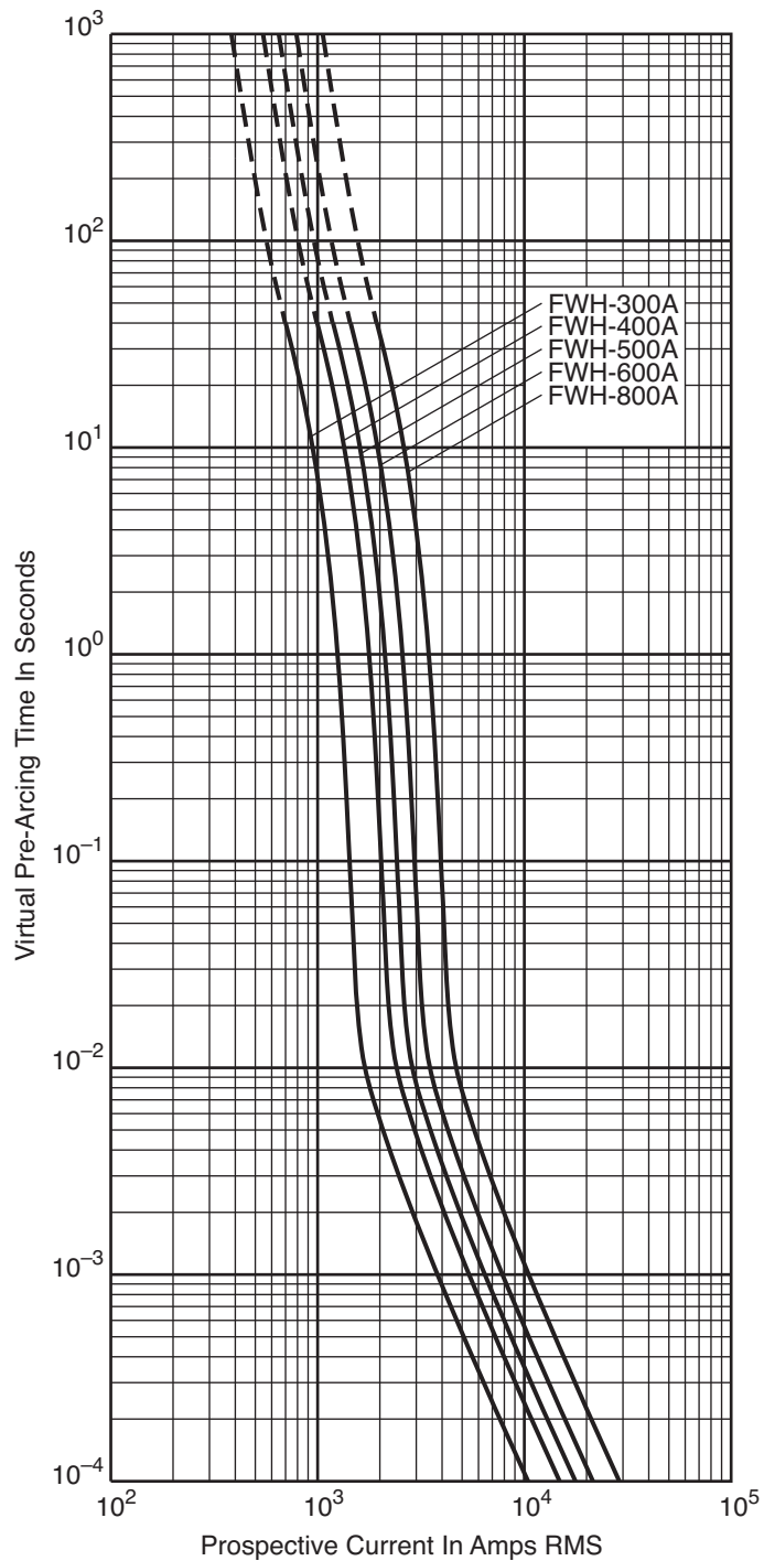
Minimum Melting, Cut-Off Current Characteristics
