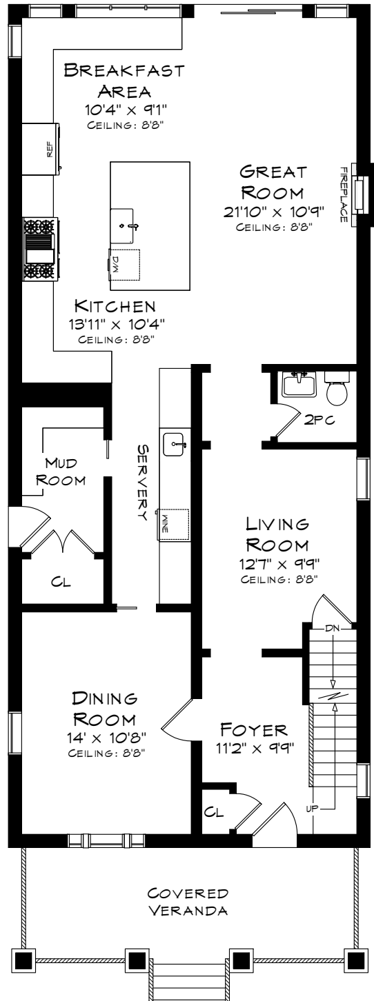
MAIN LEVEL 1,208 SQUARE FEET
