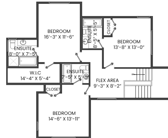
UPPER FLOOR PLAN Ceiling Height: 8'-0"
