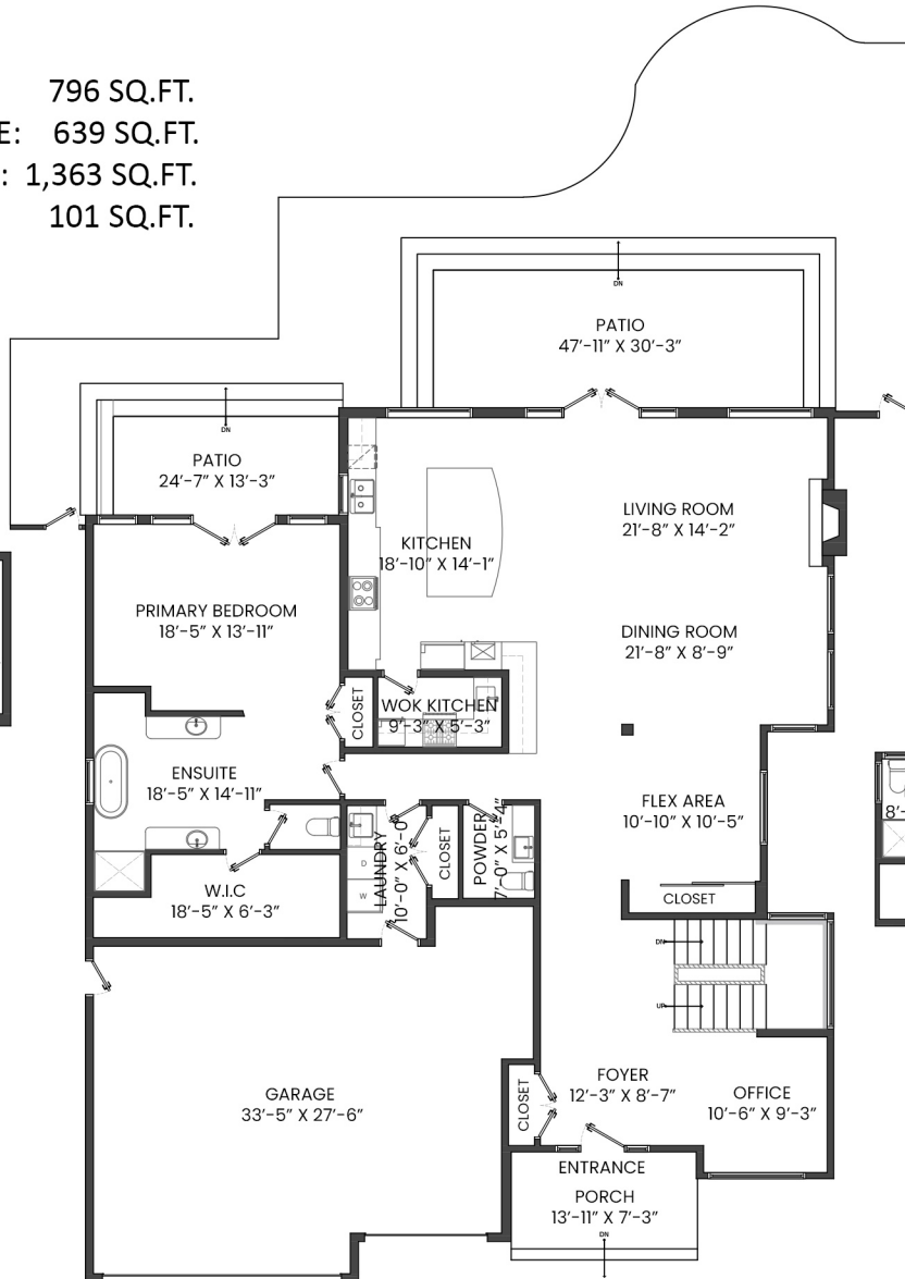
MAIN FLOOR PLAN Ceiling Height: 10'-0"
