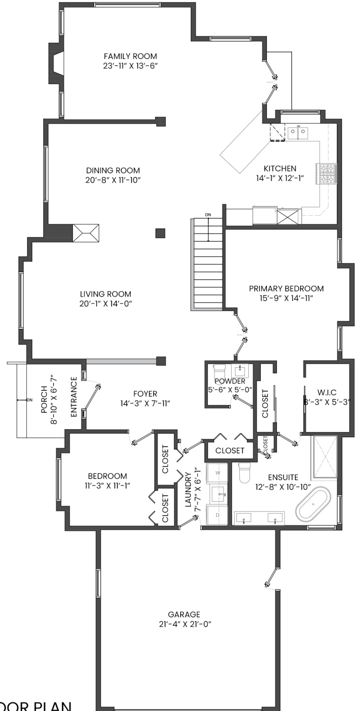
MAIN FLOOR PLAN Ceiling Height: 9'-0"
