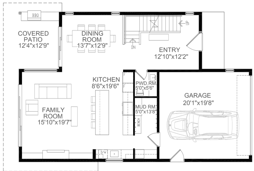
MAIN FLOOR
