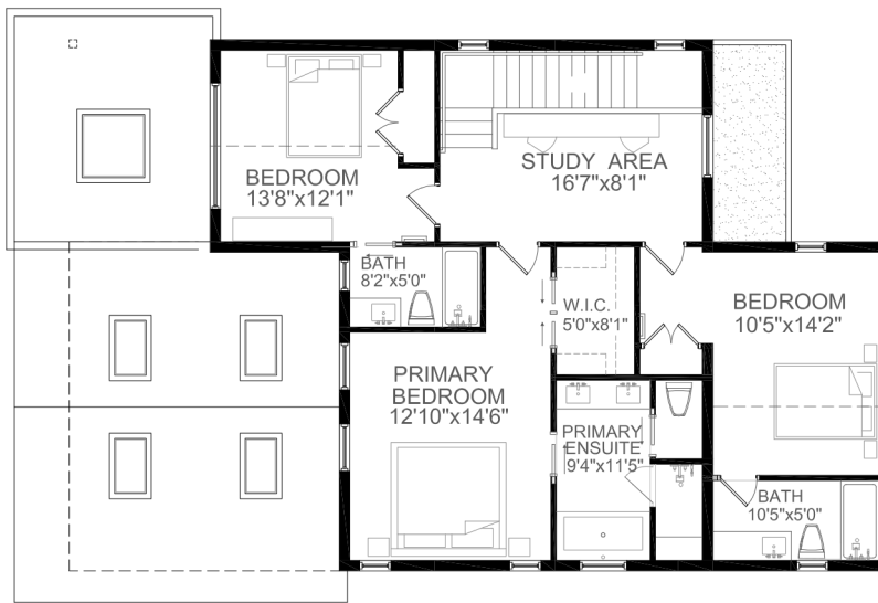
SECOND FLOOR
