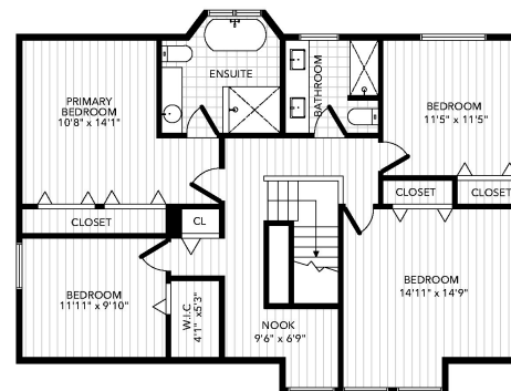
UPPER FLOOR CEILING HEIGHT: 9'
