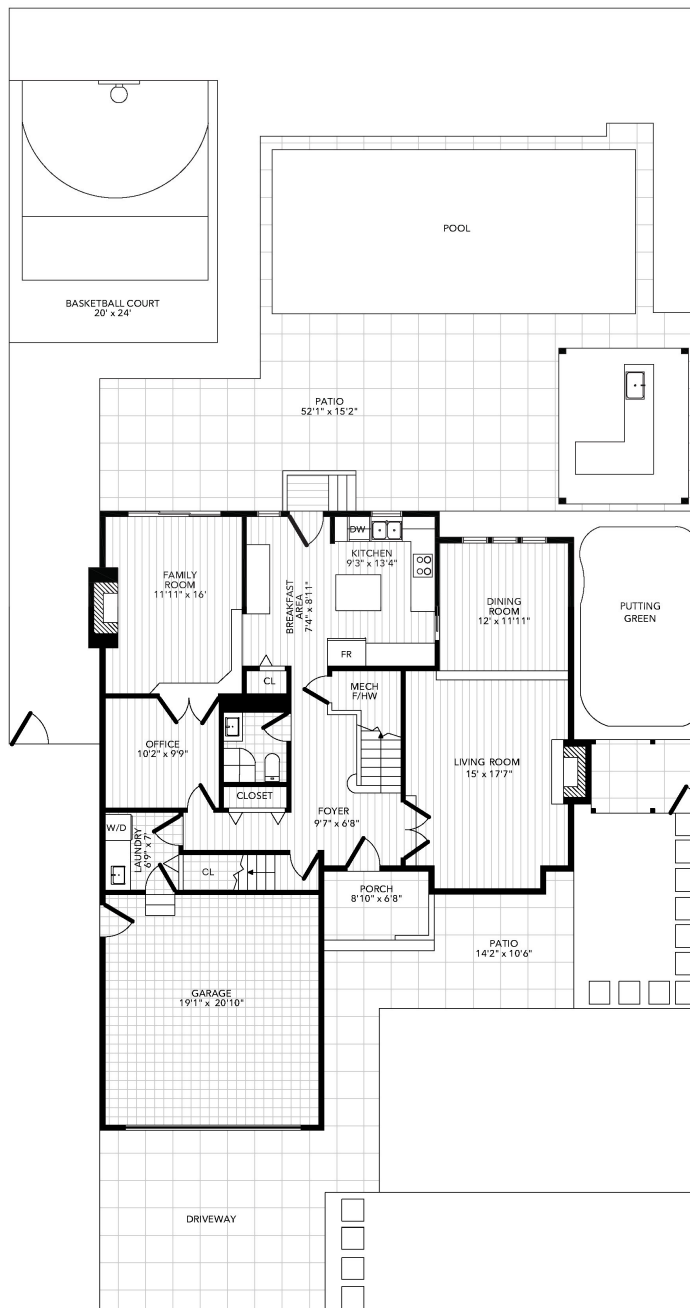
MAIN FLOOR CEILING HEIGHT: 9'
