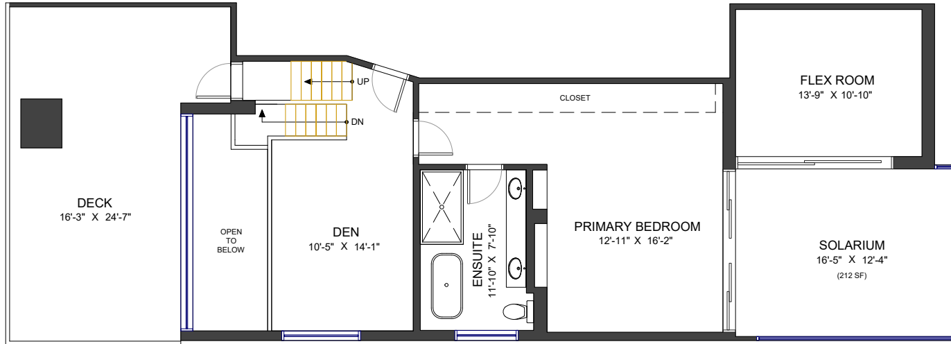
Upper Floor Ceiling Height: Max 7'-6"
