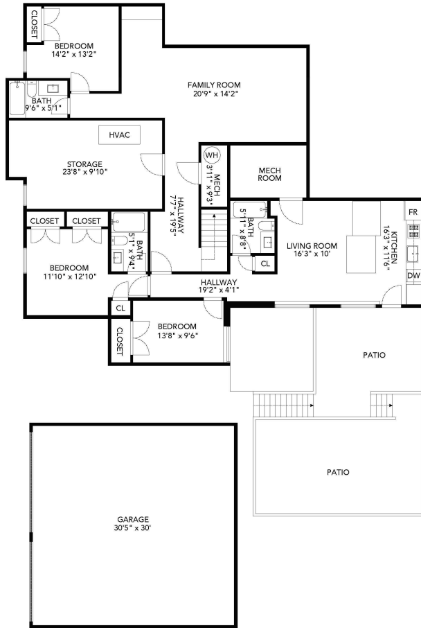
LOWER FLOOR CEILING HEIGHT: 8'
