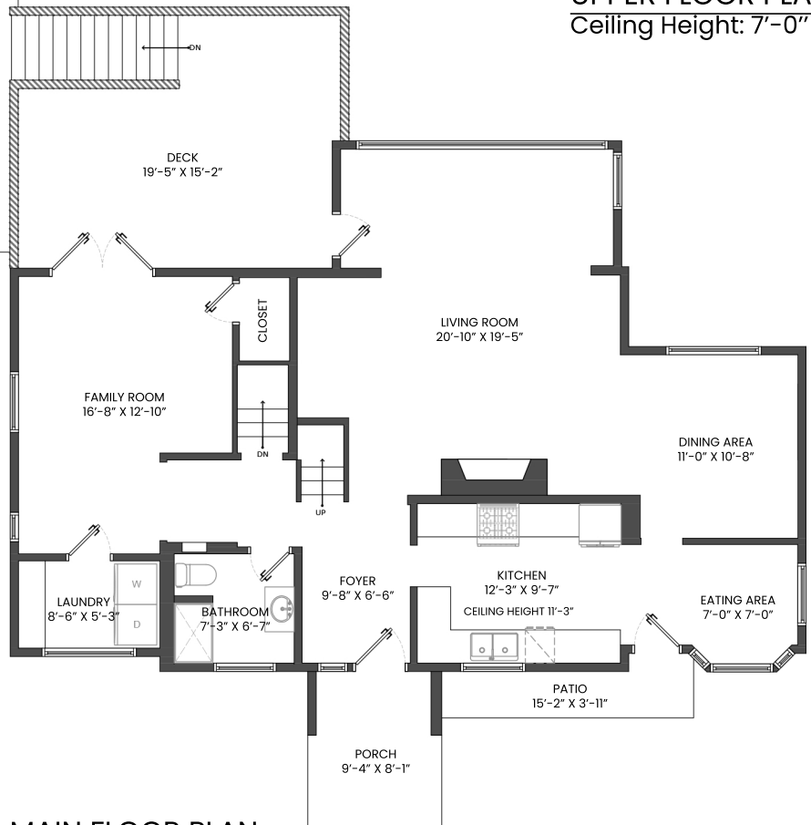
MAIN FLOOR PLAN Ceiling Height: 8'-0"
