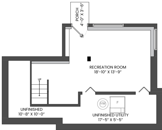
LOWER FLOOR PLAN Ceiling Height: 6'-4"
