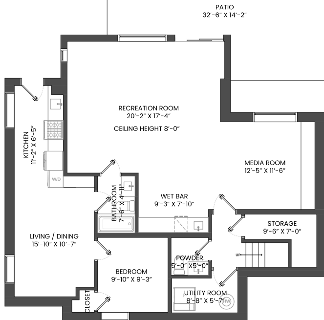
LOWER FLOOR PLAN Ceiling Height: 9'-0"
