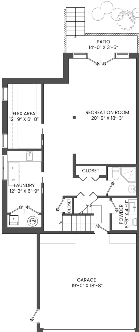
LOWER FLOOR PLAN Ceiling Height: 8'-0"
