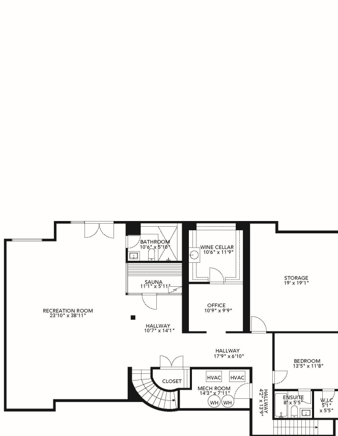
LOWER FLOOR CEILING HEIGHT: 8'3"
