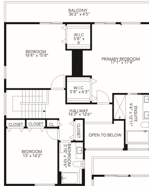
UPPER FLOOR CEILING HEIGHT: 8' ft
