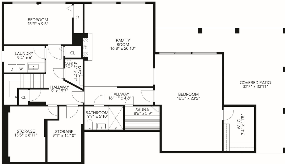
LOWER FLOOR CEILING HEIGHT: 8' ft
