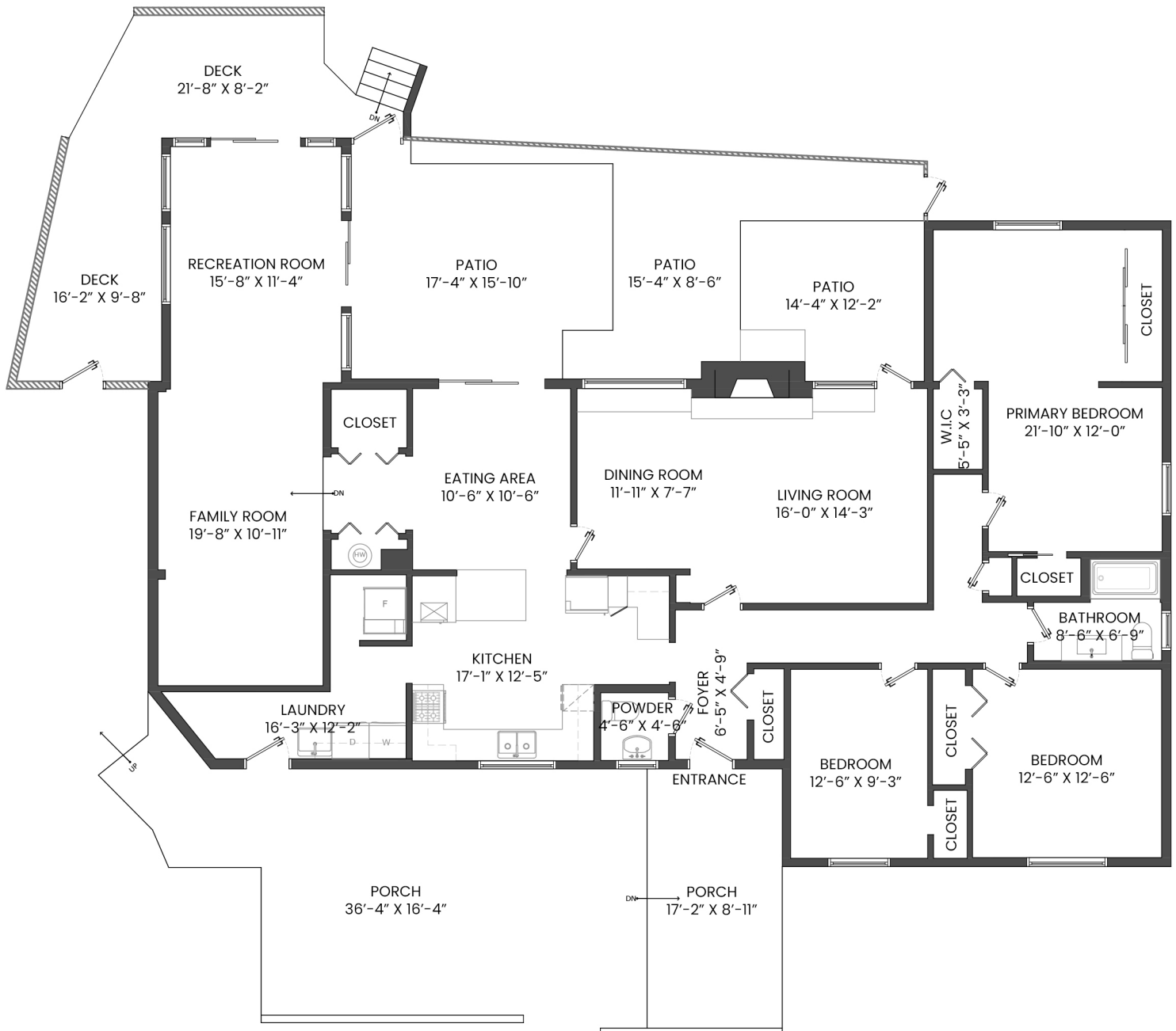
MAIN FLOOR PLAN Ceiling Height: 8'-2"
