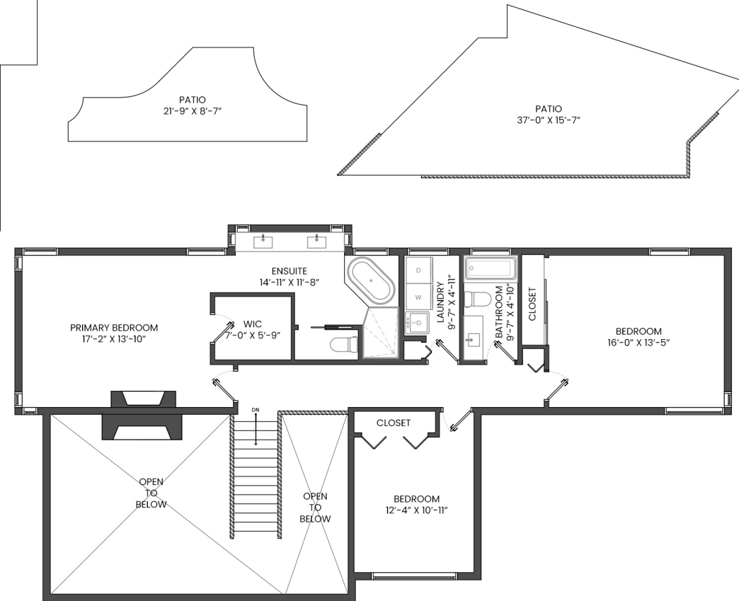
UPPER FLOOR PLAN Ceiling Height: 8'-0"
