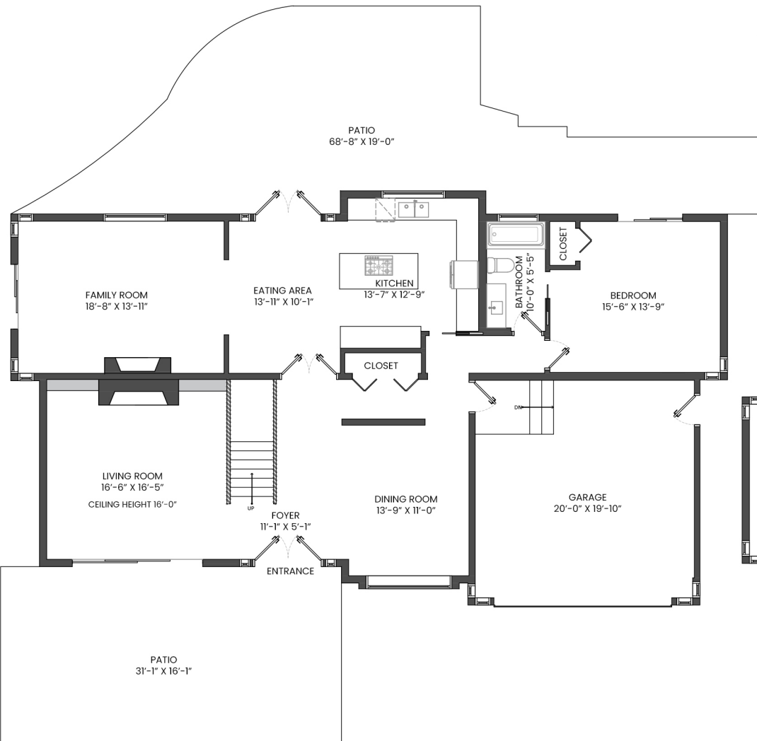
MAIN FLOOR PLAN Ceiling Height: 8'-0"
